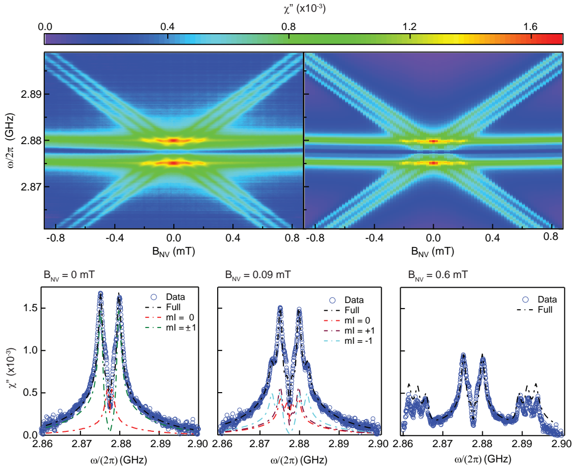
Figure 4.51: Comparison of the measured spin susceptibility with the results of numerical simulations. Measured (top left) and computed (top right) two-dimensional plots of the spin susceptibility. The bottom panel shows the spin susceptibility at B_{\text{NV}} = 0, 0.09, 0.6 mT. The dash-dotted line is the computed spin susceptibility, rescaled to match the experimental spin polarization. The computed m_I contributions to the spin susceptibility are also shown (red, purple and light blue dash-dotted lines). At B_{\text{NV}} = 0 mT, the contributions from m_I = -1 and m_I = +1 add up (green dash-dotted line).
