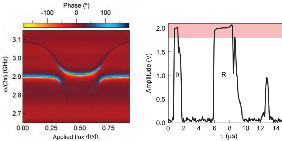
(b) Spectroscopy
