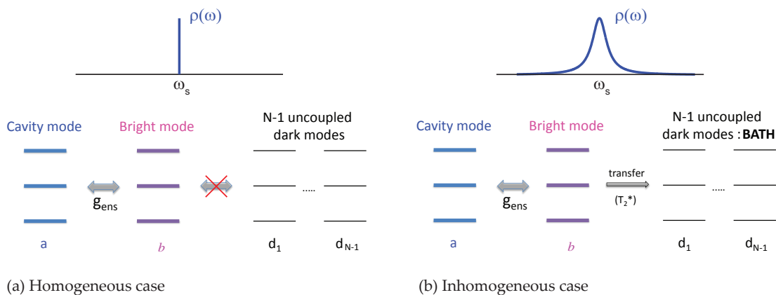
Figure 1.37: Transfer from the bright mode to the dark mode subspace enabled by inhomogeneous broadening. In the homogeneous case (a), the cavity and bright mode constitutes a closed system. The bright mode is coupled to the bath of dark modes in case of inhomogeneous broadening (b), which make it possible the transfer to the multimode dark mode subspace.
