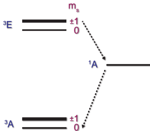
Figure 1.26: Level diagram of the NV center, showing ground ( {}^3A ) and first excited ( {}^3E ) electronic states, as well as the {}^1A state. A transition in the optical domain separates the two electronic states, which are both spin triplet ( S = 1 ).
