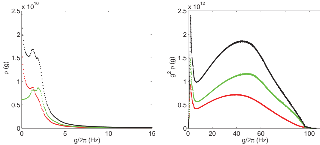
Figure 4.7: Distribution of g -parameters. The distribution \rho(g) is shown normalized as \int_0^{+\infty} \rho(g) dg = N for the N-Orth spin group (red), the Orth group (green) and for all the spins (black). A 0.7 \mu\text{m} distance between the resonator and the diamond crystal was considered for this simulation. This sets the maximum frequency cut-off observed in both graphs. (left) The distribution \rho(g) zoomed in on the low frequency part. (right) The function g^2 \rho(g) shown on the entire range of frequencies.
