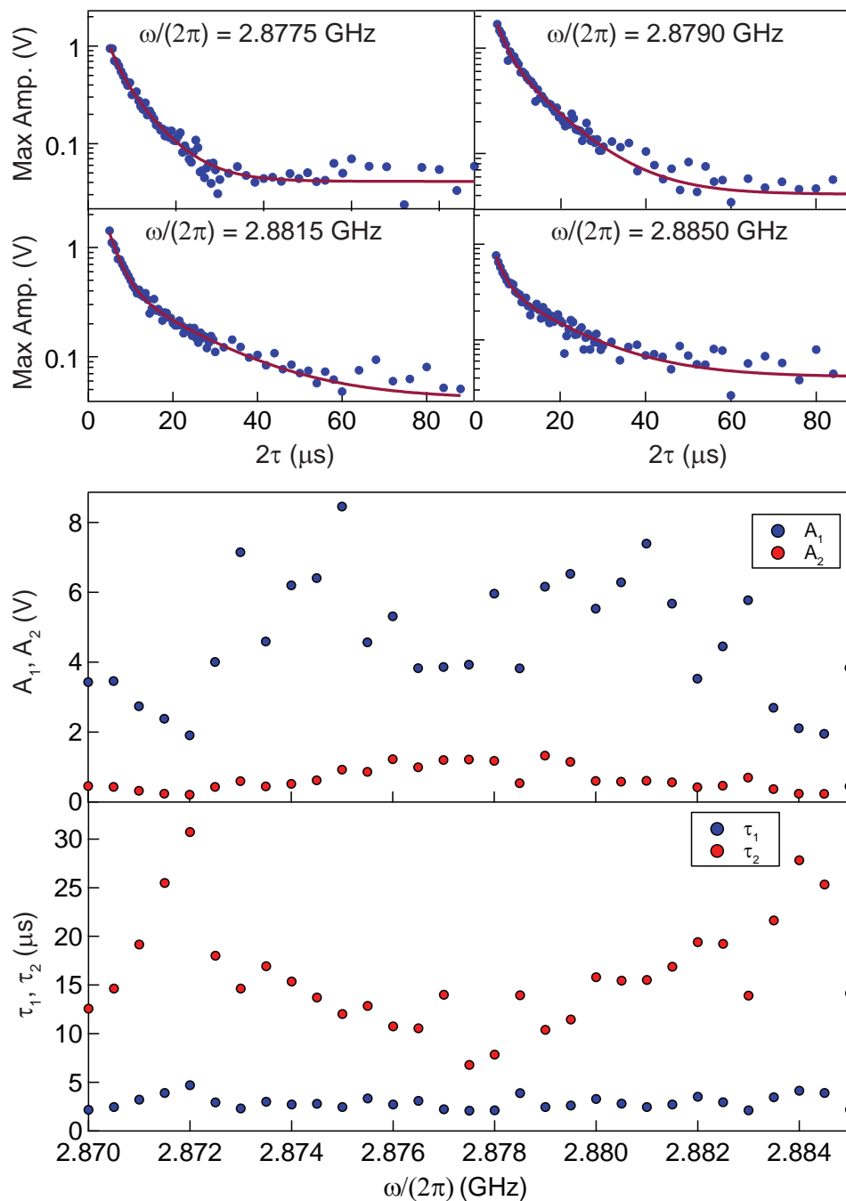
Figure 4.59: Double exponential fit of the echo decay. (top) Measured (dots) and fitted (red line) echo decay for a selection of probe frequency. (bottom) Corresponding fitted A_{1,2} and decay times \tau_{1,2} as a function of the probe frequency.
