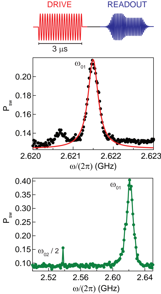
Figure 3.21: Measurement of the qubit frequency. The switching probability P_{sw} measured after a 3 \mu\text{s} drive is shown as a function of the drive frequency. Low power spectroscopy (top) shows only the |g\rangle \rightarrow |e\rangle transition of the qubit at frequency \omega_{ge} , whereas the 2-photon |g\rangle \rightarrow |f\rangle transition at frequency \omega_{gf}/2 is also observed at higher power (bottom). A Lorentzian function (red line) is fitted to the spectroscopic line at low power yielding qubit frequency \gamma_Q/2\pi = 2.6215 \text{ GHz} and linewidth \gamma_Q/2\pi = 0.13 \text{ MHz} .
