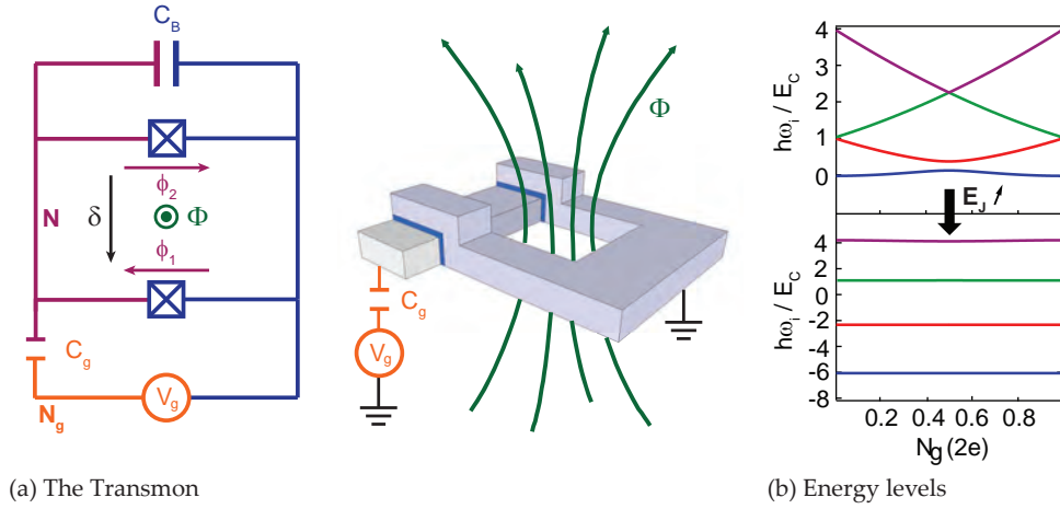
Figure 1.18: Implementation of a superconducting qubit with a Transmon. (a) The Transmon qubit used in this thesis work is a split CPB with the Josephson junction replaced by a balanced SQUID loop and (b) operated in the regime E_J \gg E_C . The first energy levels of a Transmon qubit show a charge-dispersion curve almost completely flat.
