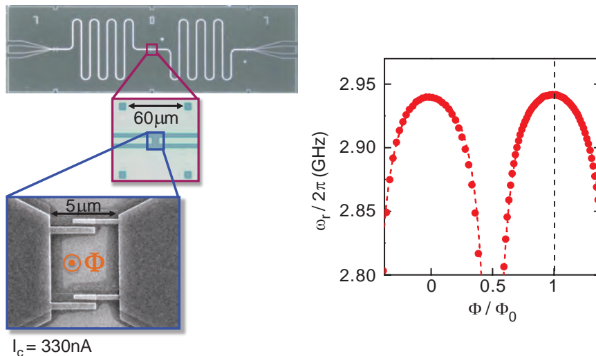
Figure 1.15: The tunable resonator. The resonance frequency of a resonator containing a SQUID is tuned by varying the flux applied to the SQUID loop.
