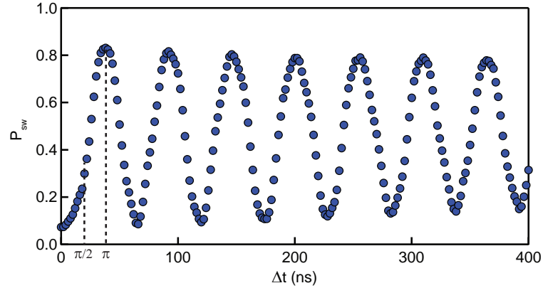
Figure 3.25: Rabi oscillations obtained for optimized qubit manipulation and readout. The optimization includes a drive with Gaussian pulse and readout with composite readout pulse.
