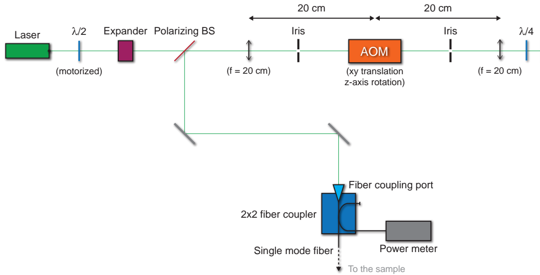
Figure 4.10: Full schematic of the optical setup. The laser beam at 532 nm passes through a half-wave plate ( \lambda/2 ) mounted on a motorized rotation stage controlled by the computer in order to choose the angle of the beam polarization. The beam is then expanded by a \times 5 expander to 4 mm and sent to the AOM through a polarizing beam splitter that selects the vertical component of the beam polarization and throw the horizontal one out of the setup (purposely to control the optical power). The beam is then focussed inside the AOM at the diffraction spot size by a convergent lens with focal length 20 cm. The angle of incidence in the AOM is adjusted with a rotation stage, on which is mounted the AOM to satisfy the Bragg diffraction condition. The first order diffracted beam out of the AOM is selected by an iris and reflects on a mirror for a second passage in the AOM. The pulsed beam is finally redirected, coupled to a single mode fiber, and splitted in two paths (90 % sent to the sample at 30 mK and 10 % to a powermeter.)
