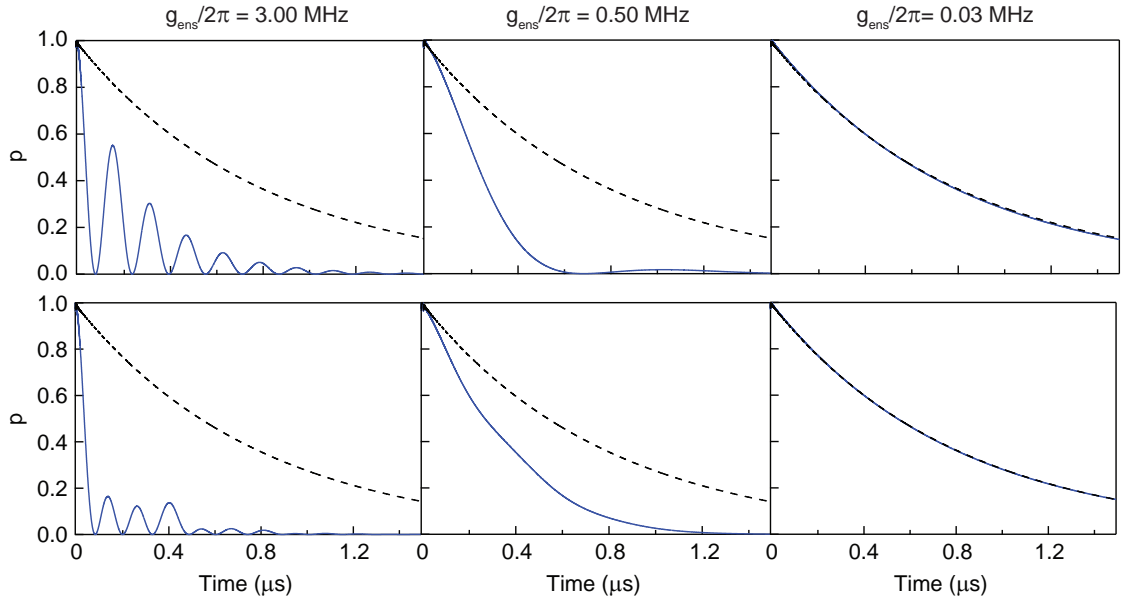
Figure 1.42: Dynamics of a photon in a resonator resonantly coupled to a distribution of spins. Probability p(t) for a single Lorentzian (top) and sum of three Lorentzian (bottom) spin distributions. The exchange of the photon is only possible in the strong coupling regime g_{\text{ens}} \gg \kappa, \Gamma . The case g/2\pi = 0 MHz that reveals the damping in the cavity alone is plotted in dashed line.
