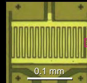
Superconducting qubits
