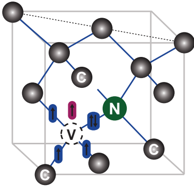
Figure 1.25: Schematic representation of the NV center in diamond.
