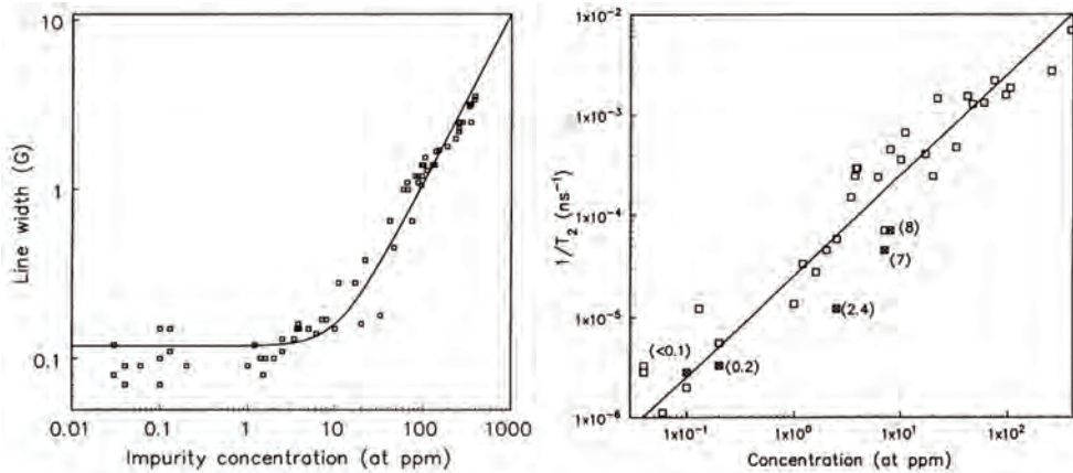
Figure 1.32: Dependence of the coherence times on the P 1 concentration [77]. Dependence of the linewidth \gamma = 1/T_2^* (left) and spin-spin relaxation rate 1/T_2 (right).
