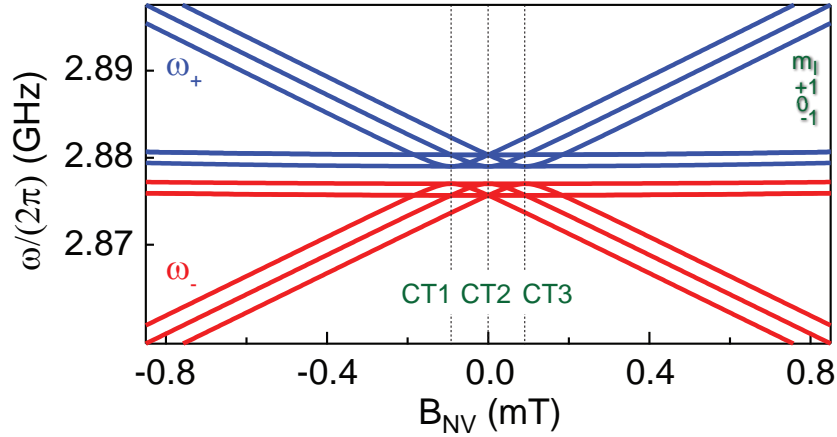
Figure 4.49: The three atomic clock transitions in NV center spins. The clock transitions are positioned at B = -B_{\text{hf}} for m_I = -1 (CT1), B = 0 for m_I = 0 (CT2) and B = +B_{\text{hf}} for m_I = +1 (CT3).
