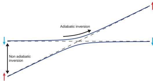
Figure 5.7: Adiabatic VS non-adiabatic inversion. The resonant inversion makes use of the Rabi oscillations of the populations, for which inversion from the initial state |\downarrow\rangle to the other state |\uparrow\rangle occurs whenever the pulse area (i.e the time-integrated Rabi frequency) equals an odd multiple of \pi , while the population returns to |\downarrow\rangle when the pulse area equals an even multiple of \pi . The adiabatic passage is based upon adiabatic following of an eigenstate of the full Hamiltonian (an adiabatic state), which links the bare states |\downarrow\rangle and |\uparrow\rangle .
