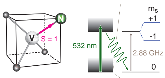
Figure 1: The nitrogen-vacancy center. Sketch of a NV center with its vacancy (V) and nitrogen atom (N), as well as three neighboring carbon atoms. Its electronic ground state has a spin S = 1 with transition between states m_S = 0 and m_S = \pm 1 at 2.88 GHz in zero magnetic field. It can be repumped optically into the |m_S = 0\rangle state.
