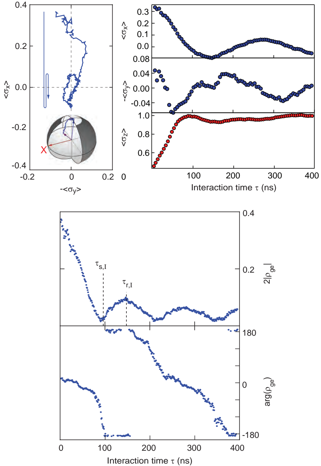
Figure 3.37: Storage of a coherent superposition of states from the qubit to the spin ensemble. (top left) Trajectory of the qubit Bloch vector on the Bloch sphere, and its projection on the equatorial plane. (top right) Components of the Bloch vector \langle \sigma_x \rangle , \langle \sigma_y \rangle and \langle \sigma_z \rangle . (bottom) Modulus and phase of the off-diagonal element \rho_{ge} of the qubit density matrix as a function of interaction time \tau .
