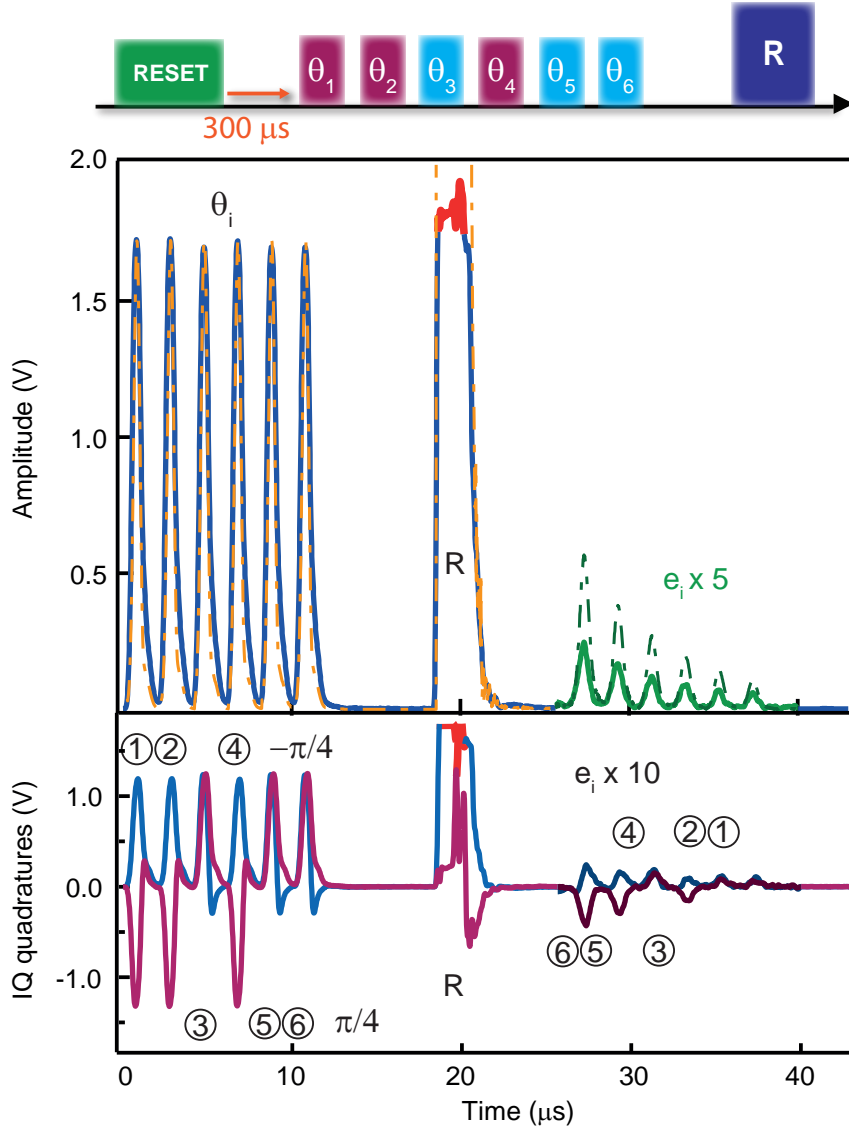
Figure 13: Read experiment. Six consecutive microwave pulses \theta_i with a varying phase and identical amplitude corresponding to \approx 10^4 photons in the resonator are absorbed by the spin ensemble, followed 10\mu\text{s} later by a strong refocusing pulse R applied to trigger their retrieval. The six pulses are recovered up to 35\mu\text{s} after their storage with an amplitude reduced by \sim 10^2 compared to the incoming pulses.
