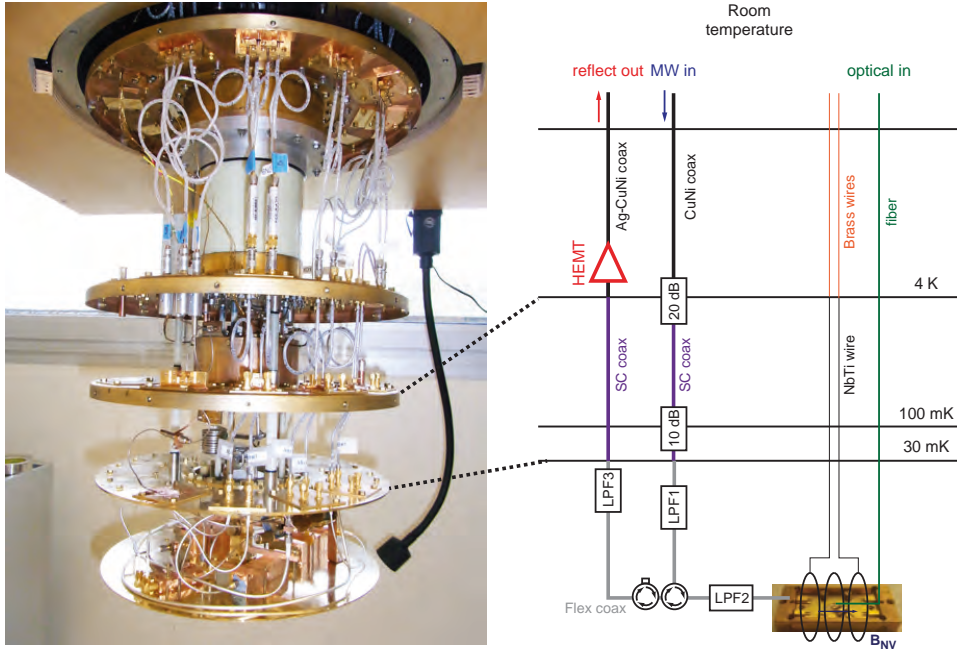
Figure 4.8: Scheme of the wiring inside the dilution refrigerator. LPF 1 , LPF 2 and LPF 3 are low-pass filters with cutoff frequencies 5.4, 4.7 and 5.4 GHz, respectively. CuNi coax is a coaxial cable made of CuNi, and Ag-CuNi coax is a silver-plated CuNi coaxial cable. SC coax is a superconducting NbTi coaxial cable. Flex coax is a low-loss flexible coaxial cable. Rectangles represent ports terminated by 50 \Omega . The cryogenic microwave amplifier is a CITCRYO 1-12 from Caltech, with gain \sim 38 dB and noise temperature \sim 5 K at 3 GHz. A DC magnetic field B_{NV} is applied parallel to the chip by passing a DC current through an outer superconducting coil. The sample box and the coil are surrounded by two magnetic shieldings consisting of a lead cylinder around which permalloy tape is wrapped. The sample box, coil, and the shieldings are thermally anchored at the mixing chamber with base temperature 30 mK (note that in the experiments using active reset of the spins with 1.47 mW laser power, the temperature was 400 mK instead).
