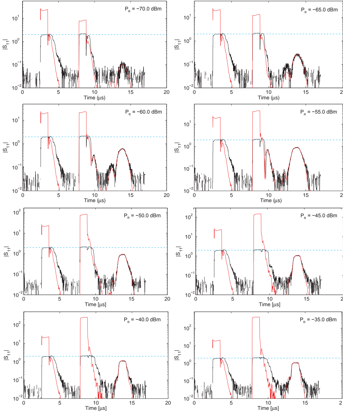
Figure 4.40: Dependence of the echo shape on the refocusing pulse power. Measured (black) and simulated (red) Hahn echo for a selected refocusing pulse power P_R . The simulations are rescaled to match the area of the echo pulses. Saturation of the amplifiers (blue dashed line) limits the measurable amplitude to about 2 V.
