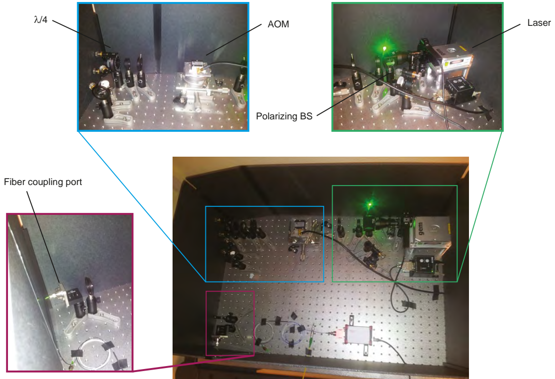
Figure 4.11: The optical setup at room temperature with panel zooming to its most important features. The laser (green panel) output a 0.8 mm diameter beam at 532 nm. Optical pulses are shape by double pass in the AOM (blue panel) and finally coupled into the single mode fiber (purple panel) that connect the setup at room temperature to the 30 mK stage.
