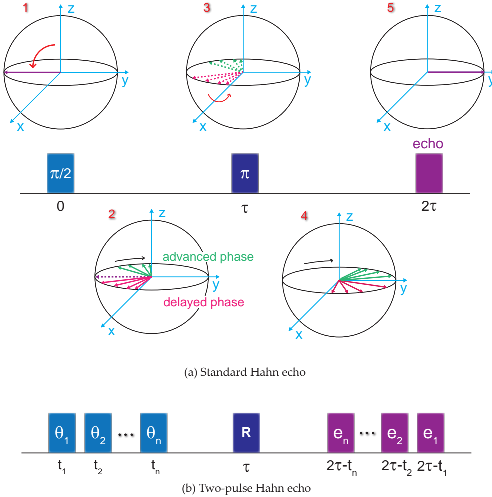
Figure 2.5: The building block of the read operation. (a) Standard Hahn echo. A \pi pulse applied at time \tau acts as a time reversal for the spins, which leads to a rephasing at time 2\tau with the emission of an echo. (b) Two-pulse Hahn echo (2PE). Weak pulses \theta_i are stored into the spin ensemble at times t_i , followed by the application of a refocusing pulse at time \tau that triggers the emission of echo pulses e_i at times 2\tau - t_i (therefore in reverse order).
