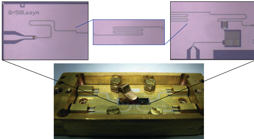
Figure 5.11: The fabricated circuit with panels zooming on its most important features. The resonator B of CPW type extends from the left to the right panels. It is designed in meanders in the middle where the diamond crystal is positioned. The resonator TF of lumped element type is visible on the right panel, with the current line used for tuning its frequency. The circuit is made in Niobium on a silicon substrate using the process described in the Appendix A. The SQUID is fabricated on top by double-angle evaporation of aluminum through a shadow mask patterned using e-beam lithography.
