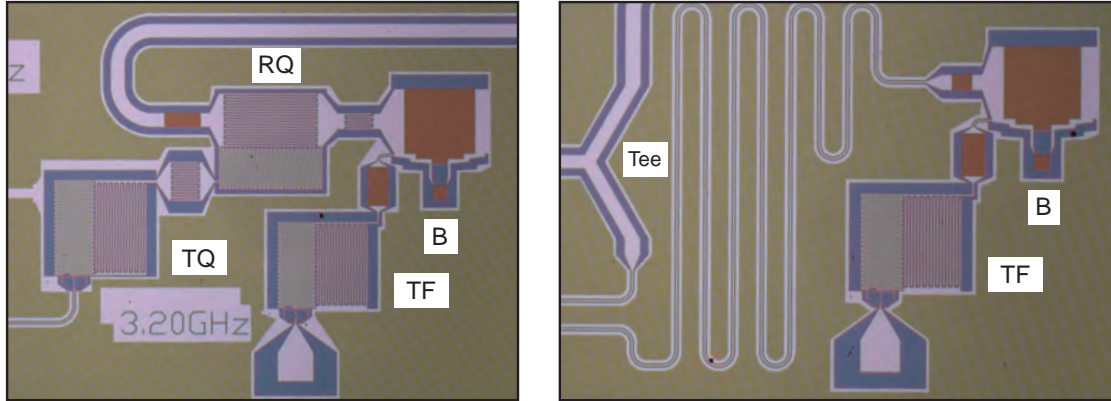
Figure 5.22: Two realizations towards a circuit able to run the full memory protocol. (left) A realization using the first approach. The design parameters are \omega_B/2\pi = \omega_{RQ}/2\pi = 2.88 GHz, \omega_{TF}/2\pi = \omega_{TQ}/2\pi = 3.20 GHz and g_{B-TF}/2\pi = g_{RQ-TQ}/2\pi = 300 MHz. A coupling capacitance C_c = 200 fF to the external measurement lines was added to set the lower limit of the quality factor of B at \sim 100 . (right) A realization using the second approach. The circuit B-TF, the tunable resonator K and the tee are patterned on a single circuit (K not shown on this picture). The design parameters are \omega_B/2\pi = 2.88 GHz, \omega_{TF}/2\pi = \omega_K/2\pi = 3.20 GHz and g_{B-TF} = 300 MHz. The coupling capacitance of B to the external measurement lines is designed to set the lower limit of the quality factor of B at \sim 200 .
