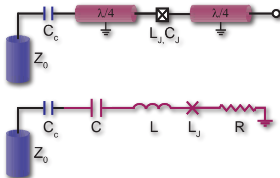
Figure 1.11: The cavity Josephson bifurcation amplifier. The CJBA fabricated in this thesis work are nonlinear, open-end \lambda/2 resonator, consisting of two sections of transmission line joined by a Josephson junction. Its equivalent lumped elements circuit is a LC resonator with capacitance C and inductance L , plus a Josephson junction with inductance L_J .
