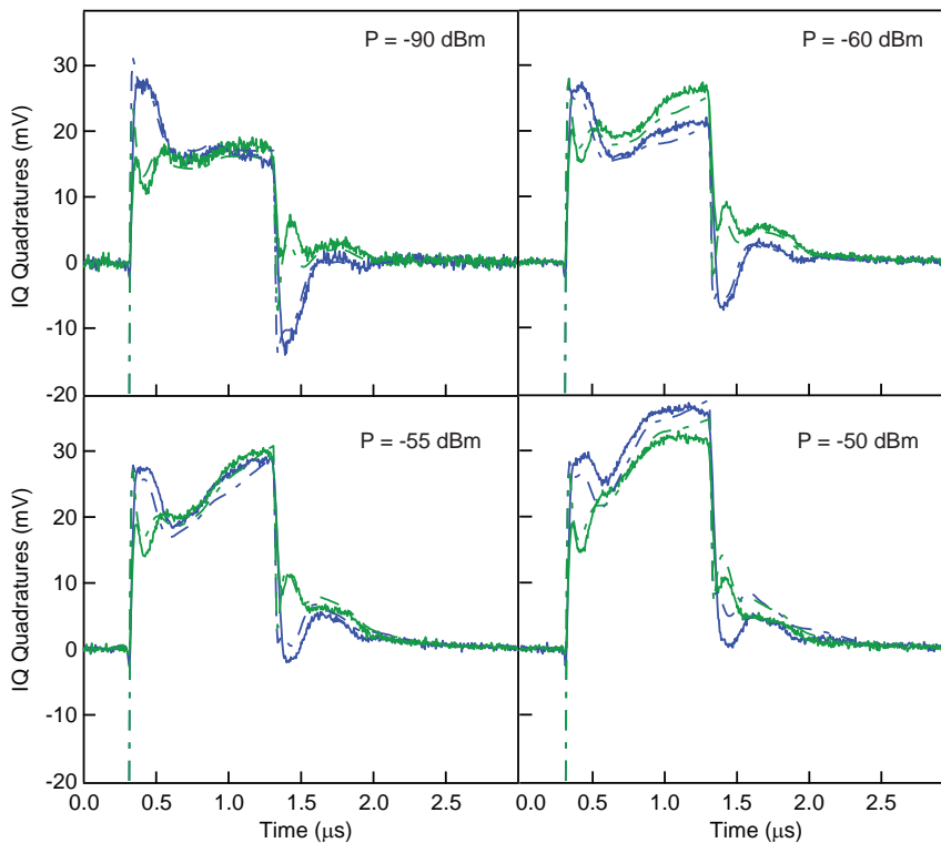
Figure 4.35: Comparison to the result of numerical simulations. In-phase (blue) and out-of-phase (green) quadratures of the reflected field for P = -90, -60, -55, and -50 dBm. The curves have been rescaled by \sqrt{P/P_0} for easier comparison, with P_0 = -90 dBm. Dash-dotted lines are simulations (see text).
