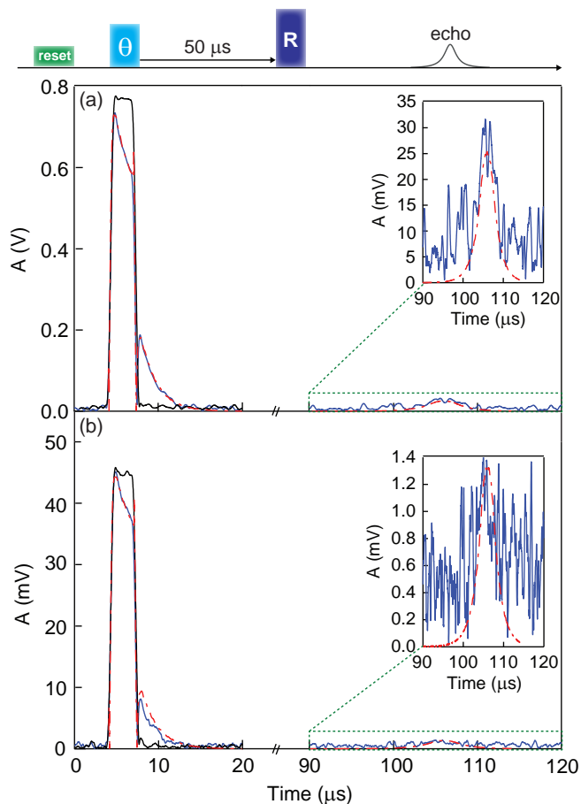
FIG. 4. Spin-echo at the few-photon level. The experimental sequence is the same as in Fig. 3, but with an initial microwave pulse having a power corresponding to (a) 60 and (b) 1 photon inside the resonator. The signal was averaged over 3 \times 10^4 (a) and 5 \times 10^5 (b) sequences, with a repetition rate of 5 Hz (a) and 10 Hz (b), limited by the laser pulse duration. Blue solid lines are experimental data, red dashed-dotted lines are the results of simulations as explained in the text.
