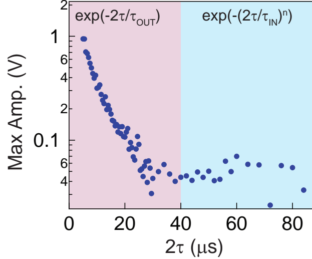
Figure 4.62: Exp+n fit . The spins OUT CT (respectively IN CT) contributes to the rapid (slow) echo decay at short (long) time as \exp(-2\tau/\tau_{OUT}) (respectively \exp(-2\tau/\tau_{IN})^n ).
