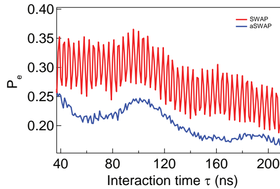
Figure 3.35: Comparison between storage using SWAP and aSWAP B-Q transfer. The probability P_e(\tau) is shown for \omega_B tuned to \omega_{-III} .
