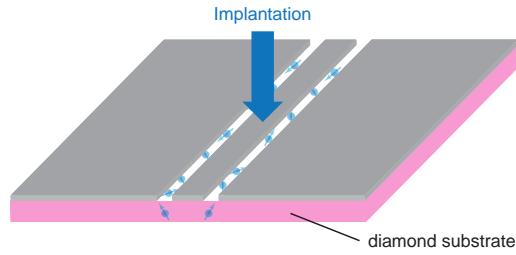
Figure 5.8: The diamond as a substrate for the superconducting circuit. The circuit is patterned on the diamond substrate and the Nitrogen atoms implanted a posteriori. A mask is placed on the superconducting layer, such that the region in which the spins are implanted is restricted to the gap between the central conductor and the ground planes.
