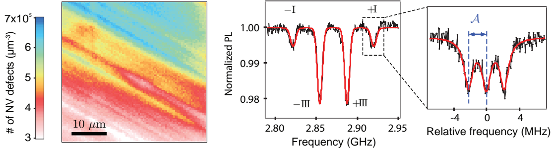
Figure 3.6: The diamond: characterization at room temperature. (left) Two-dimensional map of the NV center density for a depth of 5 \mu\text{m} inside the diamond sample. (right) Optically detected ESR spectrum with a static magnetic field B \approx 1.5 \text{ mT} applied along the [111] axis of the diamond crystal. Four ESR lines are observed, corresponding to |0\rangle \rightarrow |\pm\rangle spin transitions for the two subsets of NV centers crystalline orientations ( \pm\text{III} and \pm\text{I} ). The fit with Lorentzian functions (inset) leads to A_{\parallel} = 2.14 \pm 0.02 \text{ MHz} as expected from hyperfine interaction with ^{14}\text{N} nuclear spins.
