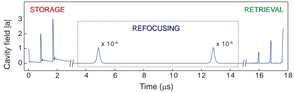
Figure 2.12: Multimode ability. The cavity field |\hat{a}| versus time in a multi-mode storage example with three input fields separated by 0.84 \mu\text{s} and memory time 16 \mu\text{s} .
