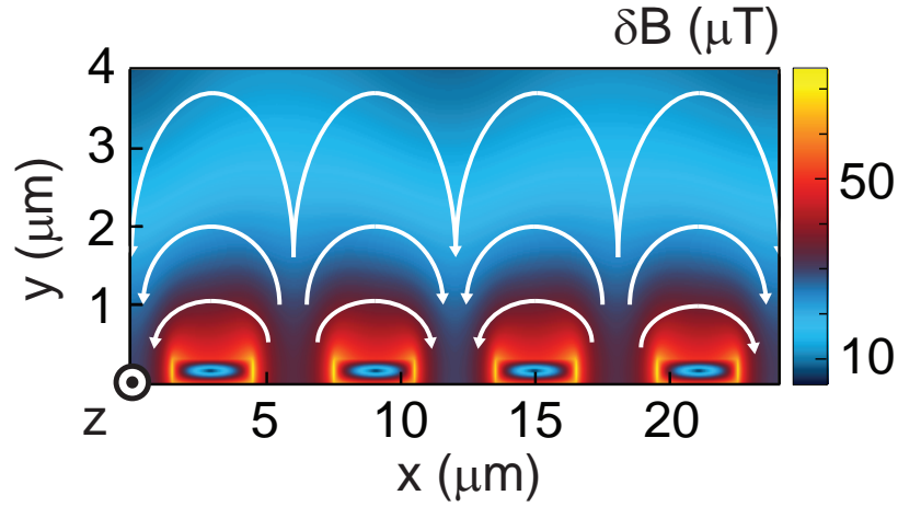
Figure 4.5: The resonator: the AC magnetic field to which the spins are coupled. Amplitude of the microwave field generated by the resonator above the inductance for a 10 \mu\text{W} incident microwave power at resonance. The field lines are superimposed on the graph.
