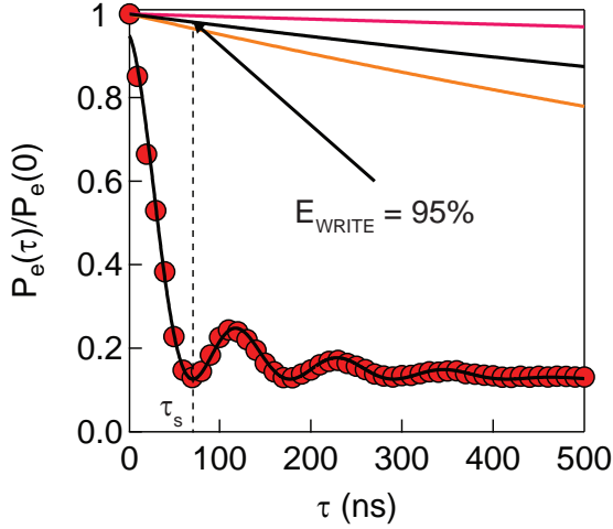
Figure 3.34: The storage efficiency. The energy relaxation in the resonator (orange) and in the spins (pink) are superimposed on the curve P_e(\tau)/P_e(0) when the bus resonator is tuned on resonance with \omega_{-III} . The efficiency of the storage process is extracted from the average of the two decays (black) as the value at full storage \tau_s over the value at \tau = 0 , yielding 95%.
