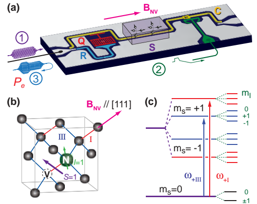
FIG. 2. (Color online) (a) Sketch of the implementation of qubit-based ESR. The spin ensemble S consists of nitrogen-vacancy (NV) centers in a diamond crystal. They are coupled to the frequency-tunable coplanar waveguide resonator C used as the ESR cavity. C also embeds the ESR-detector qubit Q , a superconducting qubit of the transmon type whose state can be read-out with another resonator R . Microwave pulses for spin spectroscopy as well as for qubit read-out are sent via an input port coupled both to C and to R . (b) and (c) Sketch and energy levels of NV centers in diamond. In our setup a DC magnetic field \mathbf{B}_{NV} is applied along the [1, 1, 1] direction, resulting in different Zeeman splittings for centers having the N - V axis parallel to \mathbf{B}_{NV} (ensemble I, in red) and those having their axis along the three other (1, 1, 1) axes (ensemble III, in blue). The ESR frequencies \omega_{\pm I, III} are further split in three resonance lines due to the hyperfine interaction with the spin-1 ^{14}\text{N} nuclear spin. 11
