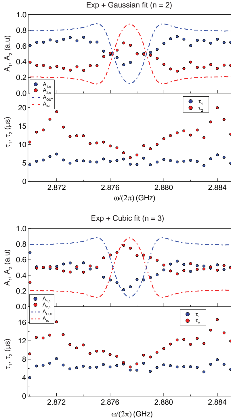
Figure 4.64: Comparison of the cases n = 2, 3 to the theory.
