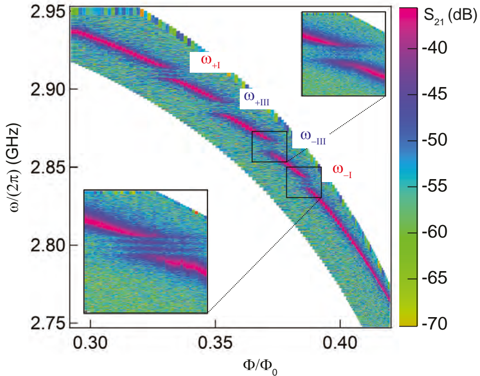
Figure 3.30: Spectroscopic evidence of strong coupling between the bus resonator and the spins. Two-dimensional plot of the transmission |S_{21}|(\omega, \Phi) through B in dB units, with \Phi expressed in units of the superconducting flux quantum \Phi_0 = h/2e , at B_{\text{NV}} = 1.4 \text{ mT} . The resonator transmission spectrum S_{21} shows four anticrossings when the bus resonator frequency crosses the NV transitions |0\rangle \rightarrow |+\rangle and |0\rangle \rightarrow |-\rangle of the two spin groups. The insets are zooms on the anticrossing at \omega_{-I} and \omega_{-III} showing the hyperfine structure due to the interaction with the spin-one nitrogen nuclei.
