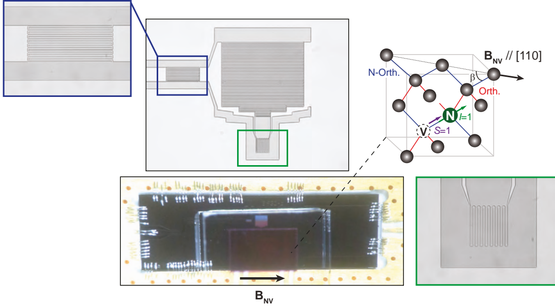
Figure 4.6: The hybrid circuit for the read experiment. The diamond crystal (dark pink) containing the NV center spins is placed on top of the resonator inductance. A spacer (transparent) is glued on the diamond top face, on which the fiber will be attached. A magnetic field B_{\text{NV}} is applied parallel to the [1, 1, 0] crystalline axis, resulting in different Zeeman splitting for centers having the NV axis orthogonal to B_{\text{NV}} (denoted Orth, in red) and those making an angle \beta = 35.3^\circ with B_{\text{NV}} (denoted N-Orth, in blue).
