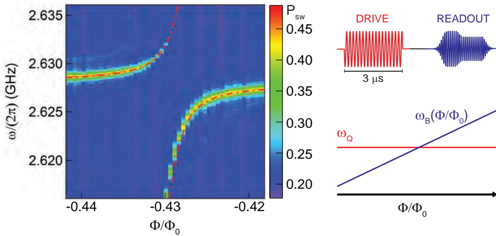
Figure 3.27: Spectroscopic evidence of strong coupling between the bus resonator and the qubit. The procedure is depicted on the right: a qubit spectroscopy is performed for increasing applied flux \Phi through the SQUID loop of the bus resonator. When \omega_B(\Phi) matches the qubit frequency \omega_Q , the qubit spectrum shows an anticrossing. The red line is a fit with the model described in Section I.1.3.1, yielding g_{B-Q}/2\pi = 7.2 MHz.
