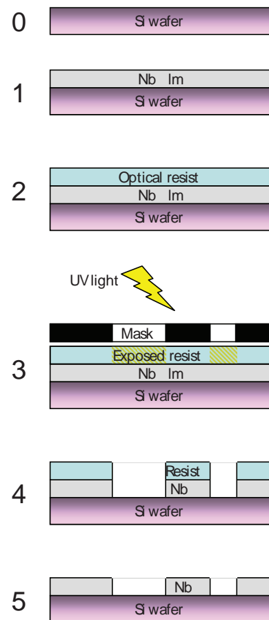
Figure 6.2: Optical lithography process.
