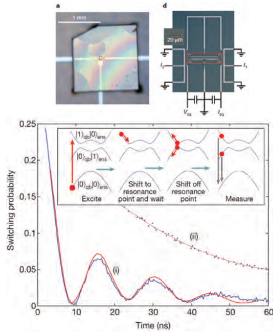
Figure 3.40: Coherent coupling of a superconducting flux qubit to an electron spin ensemble in diamond [110]. (top) Experimental set-up of the NV diamond sample attached to a flux qubit system. (bottom) Vacuum Rabi oscillations of the flux qubit/ NV^- ensemble coupled system.
