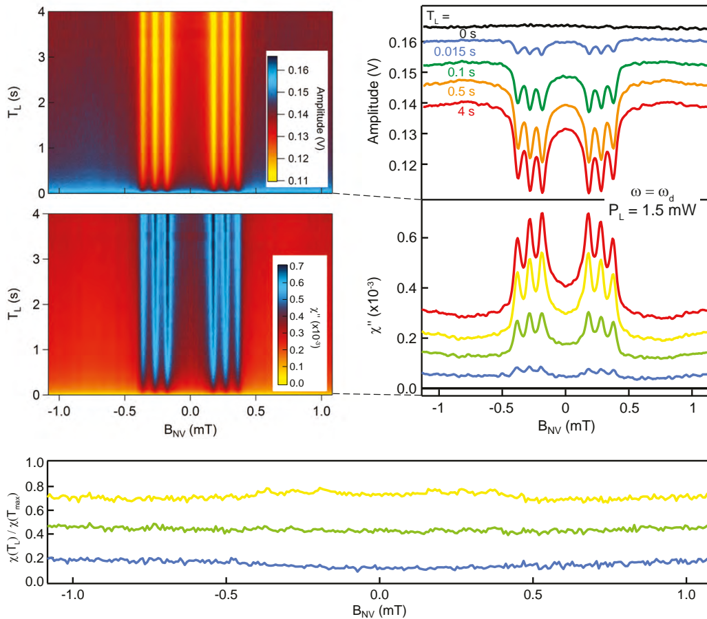
Figure 4.29: Dependence of the spin susceptibility on the optical pulse duration T_L . (top) Reflected amplitude and corresponding imaginary part of the spin susceptibility \chi''(B_{NV}) as a function of the optical pulse duration T_L for a fixed pulse power P_L = 1.47 mW. The duration T_L is swept from T_{\min} = 0 s to T_{\max} = 4 s. The left panel shows a selection. (bottom) Ratio \chi''(T_L, B_{NV})/\chi''(T_{\max}, B_{NV}) showing that the shape of the spin susceptibility \chi''(B_{NV}) is independent of the optical pulse duration.
