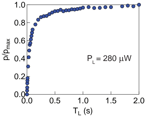
Figure 5.4: Active reset of the spins. The relative spin polarization for P_L = 280 \mu\text{W} as a function of T_L increases then saturates around T_L^{\text{sat}} = 1 s. Since P_L > P_{L,\text{max}} , the saturation corresponds to the maximum polarization allowed by optical repumping.
