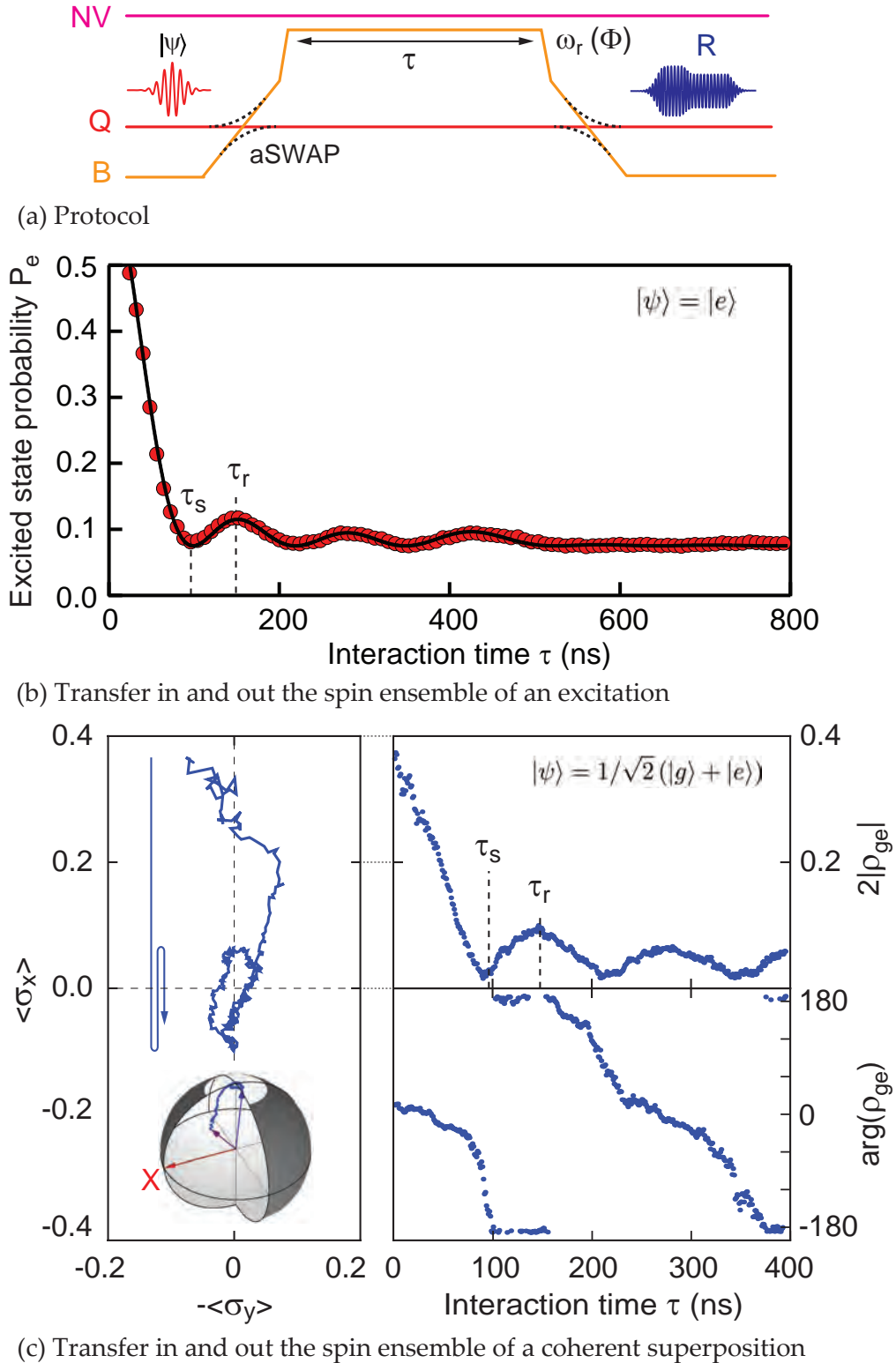
Figure 9: Write experiment. (a) Protocol for storing a qubit state into the spin ensemble. (b) Swap oscillations of an excitation |e\rangle and (c) of a coherent superposition of quantum states (|g\rangle + |e\rangle)/\sqrt{2} , initially prepared in the qubit. The transfer to the spin ensemble is complete at \tau_s .
