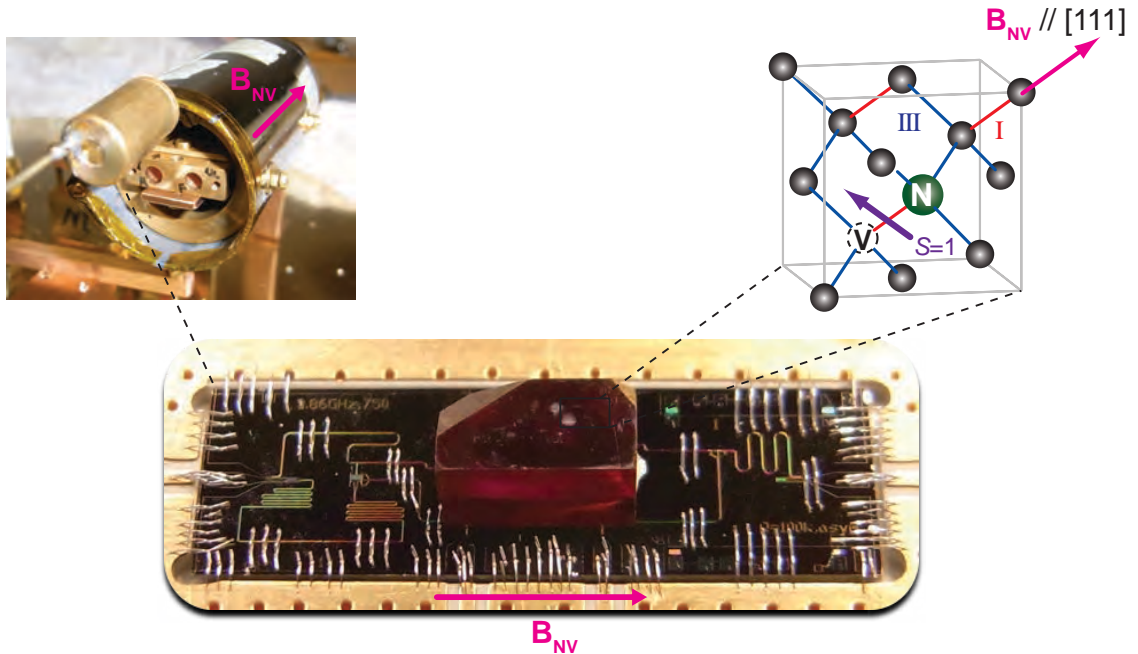
Figure 3.12: Hybrid quantum circuit for the write experiment. The diamond crystal containing the NV center spins is glued on the chip surface, in the middle of the bus resonator. A magnetic field B_{NV} is applied parallel to the [1, 1, 1] crystallographic axis, resulting in different Zeeman splittings for centers having the NV axis parallel to B_{NV} (ensemble I , in red) and those having their axis along the three other \langle 1, 1, 1 \rangle axes (ensemble III , in blue).
