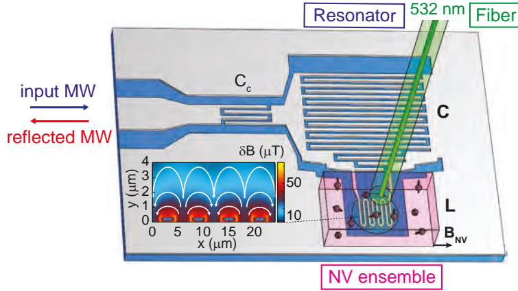
Figure 11: Read experiment: schematic of the circuit. An ensemble of NV electronic spins (pink) is coupled to a planar superconducting LC resonator. Laser pulses are shone on the diamond through an optical fiber glued to its top face, to reset the spins in their ground states between successive operation.
