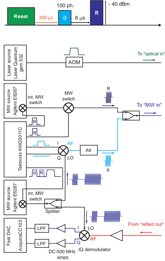
Figure 4.44: Protocol and setup for few photon pulse storage and retrieval. The local oscillator of the IQ demodulator is pulsed to suppress the refocusing pulse from the reflected signal.
