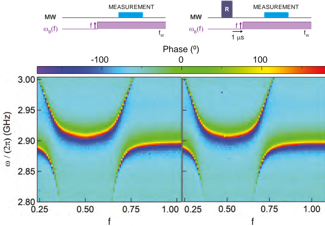
Figure 5.17: Demonstration of dynamical tuning of the resonator frequency after the refocusing pulse. (top) Experimental sequence. A strong refocusing pulse (R) is applied on resonance with B at \omega_B(f_w) , followed after a 1 \mu\text{s} delay by a fast tuning of the resonator frequency at \omega_B(f) . The circuit is measured afterwards by homodyne detection. The sequence is repeated for increasing f . (bottom) Measured reflected phase after the dynamical frequency tuning without (left) and with (right) the initial application of a strong refocusing pulse. The spectra are identical, confirming that the circuit can be detuned after the application of strong refocusing pulses.
