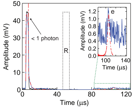
Figure 15: Storage and retrieval at the single photon level in an isotopically enriched sample having long coherence times. Less than 1 photon is absorbed by the spins and retrieved after 100 \mu\text{s} storage with 0.3 % efficiency.
