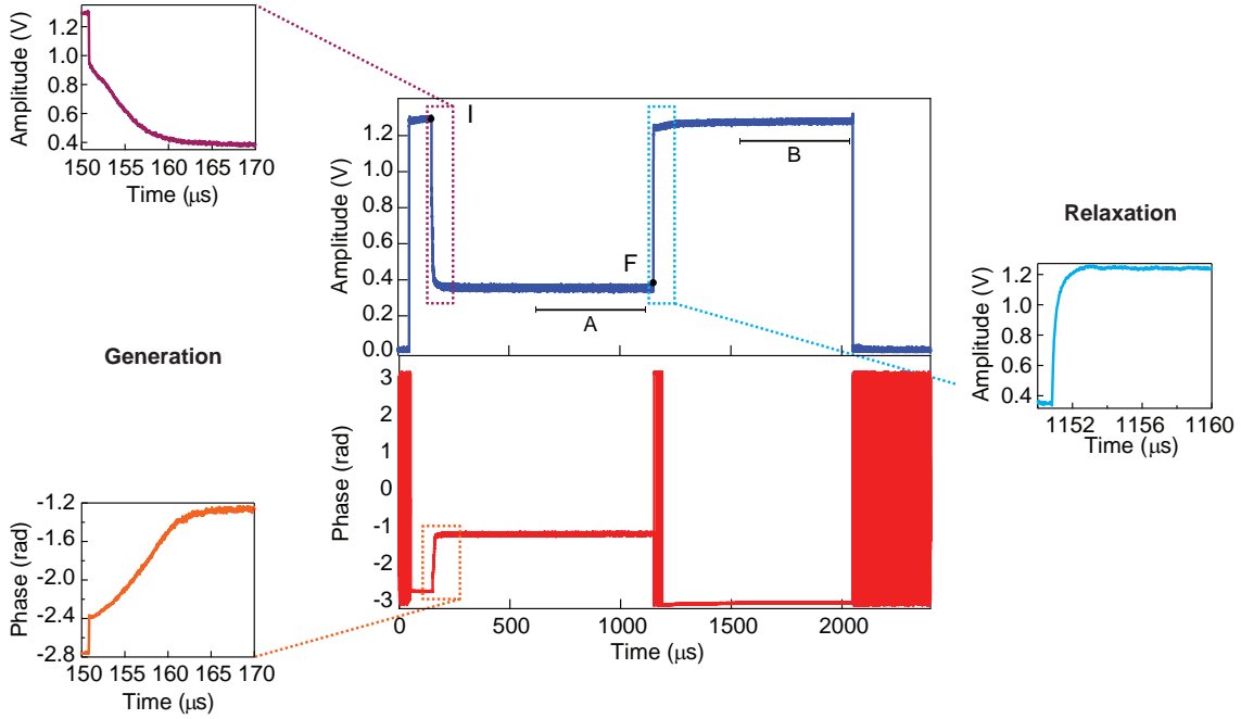
Figure 4.19: Time-domain measurement during an applied optical pulse of power P_L = 1.6 \text{ mW} , with the spins saturated. (main panel) Reflected amplitude and phase of the measurement pulse at 2.88 GHz during the application of the 1 ms optical pulse at P_L = 1.6 \text{ mW} . The spins remains saturated along the measurement. (left) and (right) are zooms on the transients which appears at the beginning and the end of the optical pulse.
