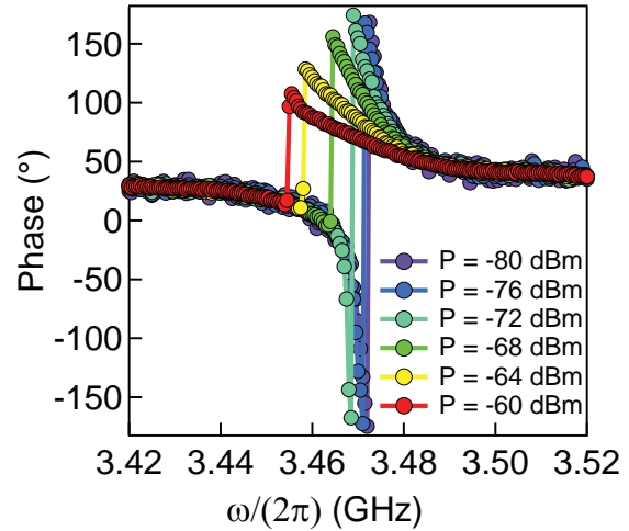
Figure 3.19: Characterization of the CJBA. The phase of the reflection coefficient for probe microwave powers P = -80, -76, -72, -68, -64, -60 dBm (from purple to red) is shown as a function of the probe frequency. The purple curve shows a \pi -shift at \omega_{\text{R}}/2\pi = 3.472 GHz, the readout resonator frequency. At powers above -72 dBm, the resonance shifts and acquires a reduced phase shift ( < \pi ) indicating that the resonator becomes non-linear. The readout parameters for qubit readout are chosen P_{\text{d}} = -64 dBm and \omega_{\text{Rd}}/2\pi = 3.458 GHz to operate in the hysteretic region of the CJBA.
