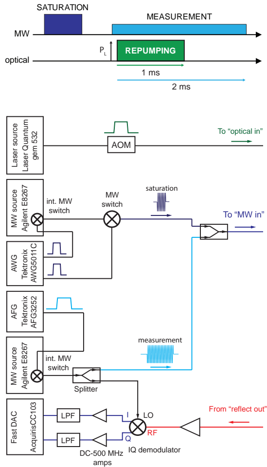
Figure 4.18: Protocol and setup for light irradiation effects measurement.
