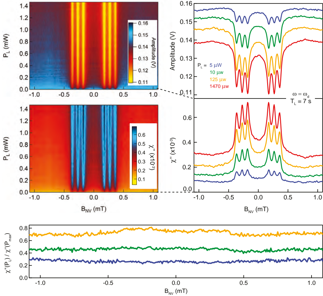
Figure 4.30: Dependence of the spin susceptibility on the optical pulse power P_L . (top) Reflected amplitude and corresponding imaginary part of the spin susceptibility \chi''(B_{NV}) as a function of the optical pulse power P_L for a fixed pulse duration T_L = 7 s. The power P_L is swept from P_{\min} = 0 mW to P_{\max} = 1.47 mW. The left panel shows a selection. (bottom) Ratio \chi''(P_L, B_{NV})/\chi''(P_{\max}, B_{NV}) showing that the shape of the spin susceptibility \chi''(B_{NV}) is independent of the optical pulse duration.
