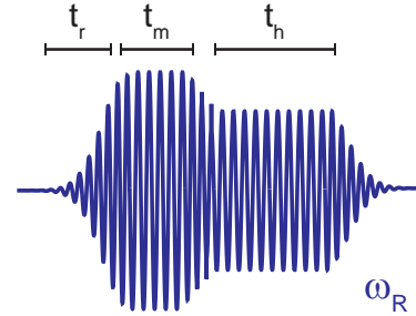
Figure 3.16: The readout pulse. The microwave signal at frequency close to \omega_R is modulated by a complex shape with 3 characteristic times. The pulse rises linearly in a time t_r similar to the resonator rise-time \kappa^{-1} , is maintained during t_m in the vicinity of the bifurcation point \beta_+ to let the transition of the resonator \bar{\mathbf{B}} \rightarrow \mathbf{B} occurs and finally hold for at time t_h at slightly lower power for measurement.
