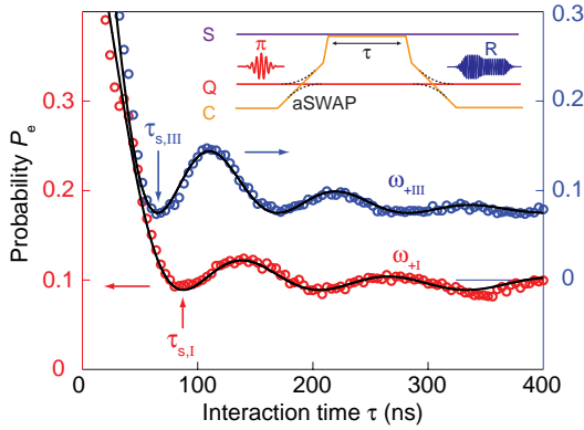
FIG. 3. (Color online) Single photon transfer between qubit and spins (Ref. 9). (inset) Pulse sequence used to excite the qubit in state |e\rangle and transfer its excitation to S via C back and forth. (panel) Swap oscillations for the two spin frequencies \omega_{+I} and \omega_{+III} . Swap times \tau_{s,I} and \tau_{s,III} are indicated by arrows. Note that the two curves are shifted vertically for clarity with corresponding scales on the left (for ensemble I) and the right axes (ensemble III).
