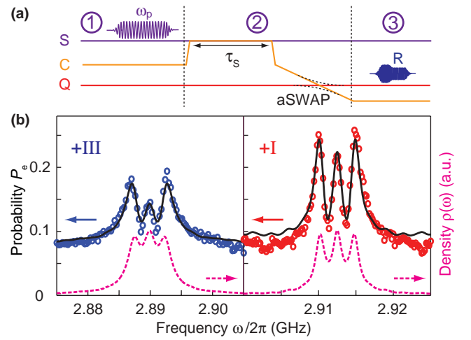
FIG. 4. (Color online) (a) Experimental pulse sequence used for qubit-detected ESR: (1) The spins are first weakly excited by a 2\ \mu\text{s} microwave pulse with a frequency \omega_p ; (2) the resulting spin excitation is transferred to the cavity C by a fast flux pulse, which brings \omega_c in resonance with \omega_K ( K = +I, +III ) for a swap time \tau_{s,K} , and then to the qubit Q by an adiabatic swap (aSWAP). (3) The qubit excited state probability P_e is finally measured. (b) Measured (open circles) and calculated (solid line) P_e(\omega_p) for spin ensemble +III (left) and +I (right). The spin density \rho(\omega) used in the calculation is shown as a dashed line.
