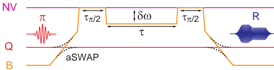
Figure 3.38: Protocol for Ramsey-like experiment on the spin ensemble at the single-photon level. The sequence shows the microwave pulses used for exciting the qubit in |e\rangle (red) and for reading it out (blue), as well as transition frequencies of the quantum bus (orange), qubit (red), and spins (magenta). B is then detuned from the spins by \delta\omega/2\pi = 38 MHz during a time \tau .
