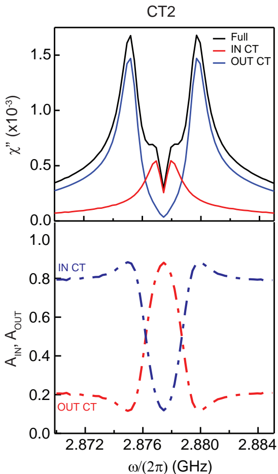
Figure 4.57: Theoretical predictions at CT 2 . (top) IN and OUT CT contributions to the spin susceptibility. (bottom) Corresponding A_{\text{IN}} and A_{\text{OUT}} weights.
