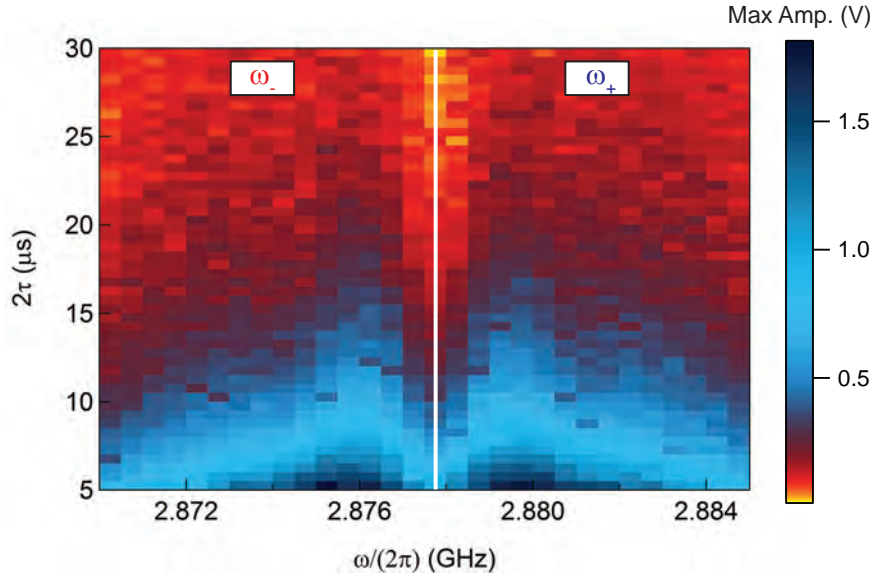
Figure 4.58: Dependence of the echo decay on the probe frequency at B_{CT2} . Two peaks are visible, corresponding to the spin transitions |0\rangle \rightarrow |\pm\rangle .
