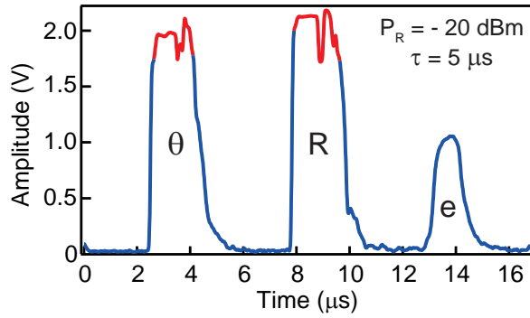
Figure 4.38: Hahn echo at high power. The echo ( e ) is observed at time 2\tau . Saturation of the amplifiers (shown in red) limits the measurable amplitude to about 1.8 V.
