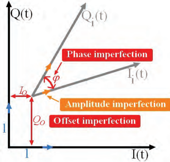
Figure 3.18: IQ mixer calibration. The correction for the IQ mixer imperfections is represented in the complex domain, with the IQ basis without calibration (in grey), and the orthogonal IQ basis obtained with calibration (in black).
