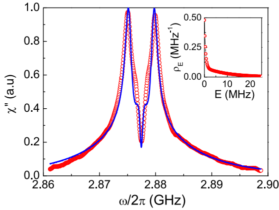
Figure 4.17: Rescaled spin susceptibility \chi''(\omega, B_{\text{NV}} = 0) . Open red circles are experimental data, solid blue line is the theory computed with the bi-exponential strain distribution \rho_E(E) shown in the inset, with a Lorentzian \rho_b(b) and \rho_D(D) with respective widths dB_0 = 0.21 \text{ Gs} and dD_0/2\pi = 150 \text{ kHz} .
