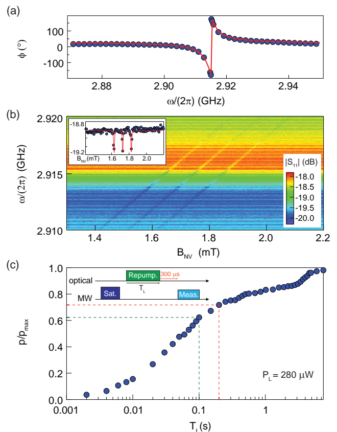
FIG. 2. (a) Phase \phi of the resonator reflection coefficient S_{11}(\omega) measured with a vector network analyzer (blue dots), yielding \omega_r/2\pi = 2.915 GHz and Q = 650 (red line is a fit to the data). (b) S_{11}(\omega) as a function of B_{NV} around 1.8 mT, showing the NV centers as a triplet of absorption dips. The inset shows |S_{11}|(B_{NV}) at \omega/2\pi = 2.915 GHz; blue dots are data, and red line is a fit to a sum of three Lorentzians with linewidth 0.012 mT. (c) Measured spin polarization for a laser pulse of power P_L = 280 \mu\text{W} as a function of its duration T_L , renormalized to its maximal value. Dashed red and black lines indicate the laser pulse durations T_L = 0.2 and 0.1 s used in the experiments shown in Figs. 3 and 4, corresponding to relative polarizations p/p_{max} = 0.72 and 0.62 .
