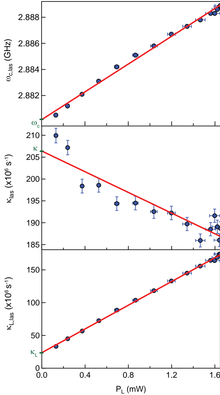
Figure 4.21: Parameters of the resonator under optical irradiation. Resonator frequency \omega_{r,laser} (top), damping rate \kappa_{laser} (middle) and internal losses \kappa_{L,laser} (bottom) as a function of the optical power P_L . The origin of the linear fit (red lines) gives a precise measurement of the resonator parameters without optical irradiation.
