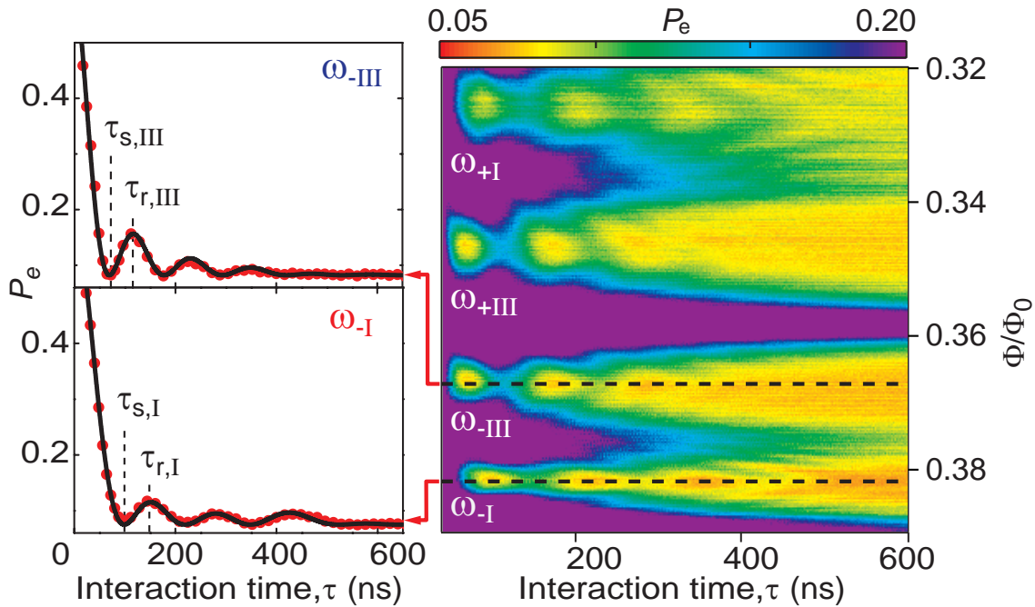
Figure 3.33: Storage of a single quantum of excitation from the qubit to the spin ensemble. (left) Experimental (dots) and theoretical (dash-dotted line) probability P_e(\tau) for \omega_B tuned to \omega_{-III} (top graph) or \omega_{-I} (bottom graph), showing the vacuum Rabi oscillation between the bus resonator and the spin ensemble. (right) Two-dimensional plot of P_e versus interaction time \tau and flux pulse height \Phi , showing resonance with the four spin groups. Chevron-like patterns are observed, showing a faster oscillation with reduced amplitude when \omega_B is detuned from the spin resonance, as expected. Note that the difference between the \omega_{-} and \omega_{+} patterns in the same NV group is simply caused by the non-linear dependence of \omega_B on \Phi [35].
