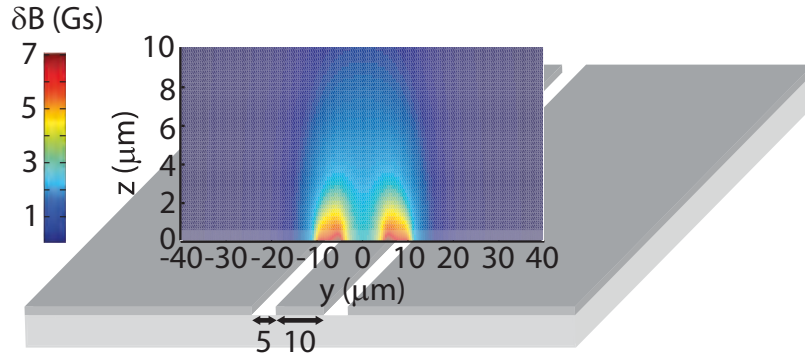
Figure 3.10: The bus resonator: the AC magnetic field to which the spins are coupled. Amplitude of the microwave field generated by the bus resonator driven at resonance by an incident microwave of power 1 \mu\text{W} .
