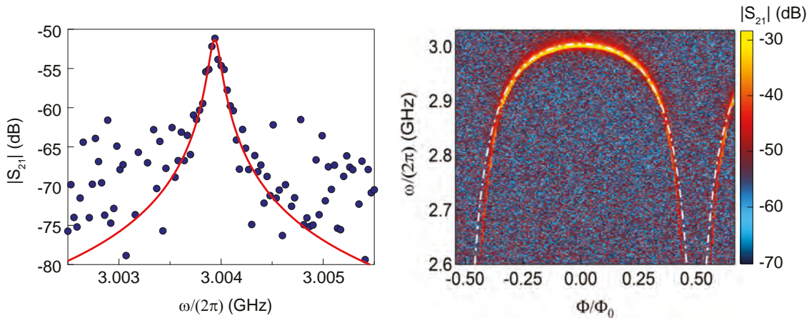
Figure 3.26: Characterization of the bus resonator. (left) Resonance line of the bus resonator at \Phi = 0 (dots). The line is a fit with a Lorentzian. (right) Two-dimensional plot of the resonator spectrum as a function of the applied flux \Phi . The fit (white dash-dotted line) yields a SQUID critical current 2I_{c0} = 1.3 \mu\text{A} .
