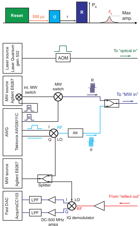
Figure 4.37: Protocol and setup for Hahn echo at high power.
