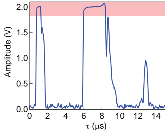
Figure 5.16: Hahn echo at f_W . A 0.5 \mu\text{s} microwave pulse ( \theta ) with power -68.5 dBm is applied creating a transverse magnetization in the spin ensemble, followed 6 \mu\text{s} later by a 2 \mu\text{s} refocusing pulse ( R ) with power -30.5 dBm. The echo ( e ) is observed at time 2\tau , confirming that the circuit is not affected by the application of strong refocusing pulses. Saturation of the amplifiers (shown in red) limits the measurable amplitude to about 1.8 V.
