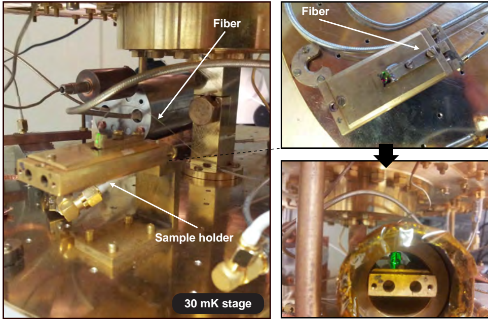
Figure 4.9: The 30 mK stage. The optical fiber guides light down to the sample at 30 mK, and is glued on it after alignment.
