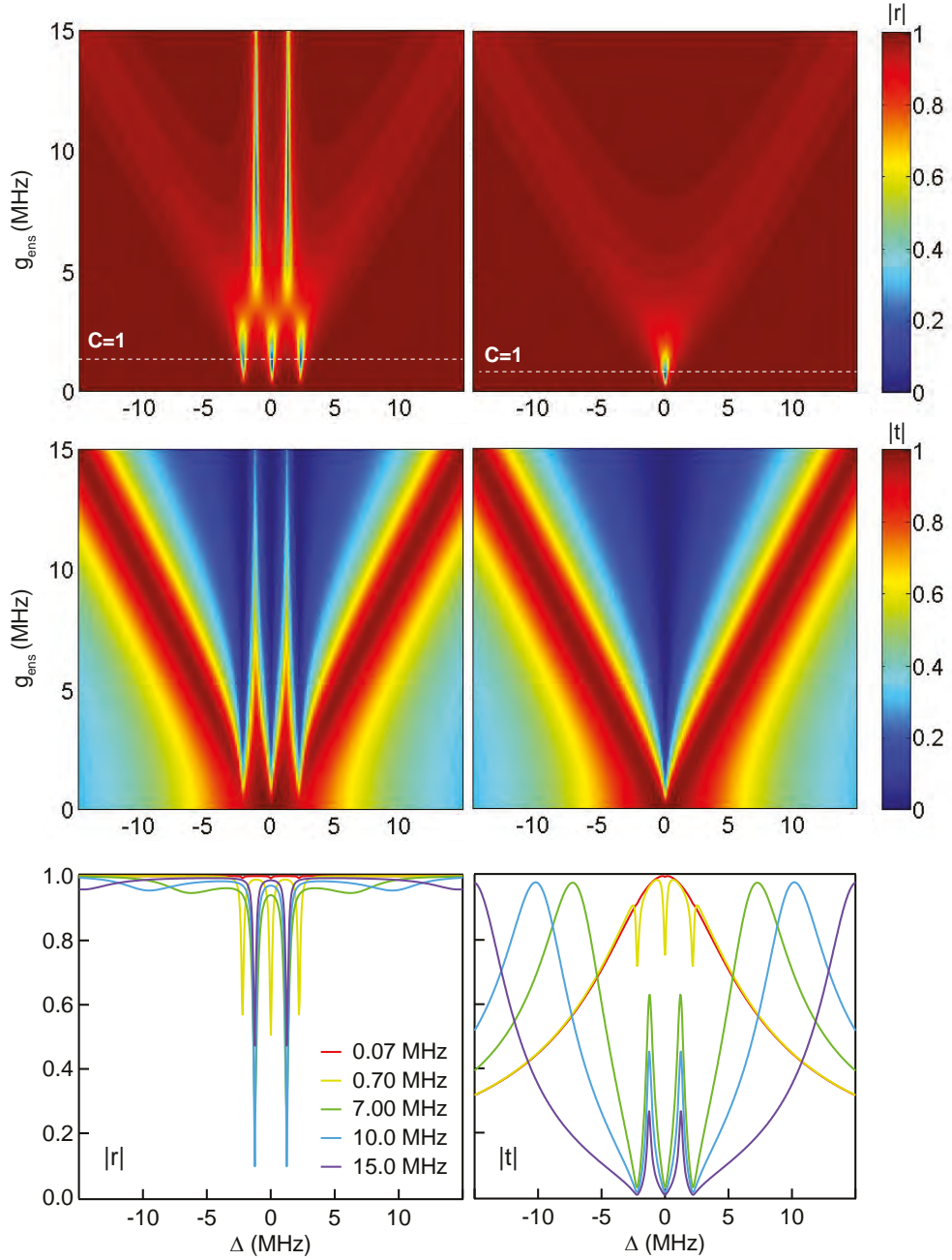
Figure 1.41: Reflection and transmission of a resonator resonantly coupled to a distribution of NV center spins. Case \Gamma/(2\pi) = 0.1 MHz and \kappa/(2\pi) = 10 MHz. The same condition for the single Lorentzian distribution is shown on the right for comparison. In the bottom panel, the graphs for g_{\text{ens}}/2\pi = 0.07 MHz (red), 0.7 MHz (yellow), 7 MHz (green), 10 MHz (light blue) and 15 MHz.
