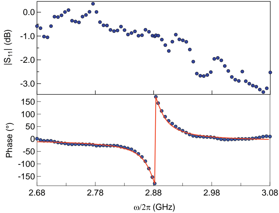
Figure 4.15: Reflection coefficient S_{11} of the resonator. The amplitude and phase reflected onto the resonator is shown when the spins are saturated and do not contribute to the signal. The fit of the phase response (red line) yields resonator frequency \omega_r/2\pi = 2.88 GHz and quality factor Q = 80 \pm 8 . The effect of spurious resonances in the measurement setup is visible in the amplitude signal.
