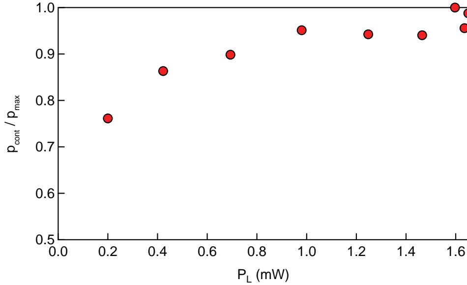
Figure 4.26: Spin polarization under continuous optical irradiation p_{\text{cont}}(P_L)/p_{\text{max}} . The spin polarization increases exponentially with P_L with characteristic power P_{L,\text{cont}} = 0.45 \text{ mW} and reaches the maximum allowed by optical repumping p_{\text{max}} \sim 90\% . The optical pumping is dependent on the optical power P_L due to a weak excitation by thermal photons that counteracts the repumping process.
