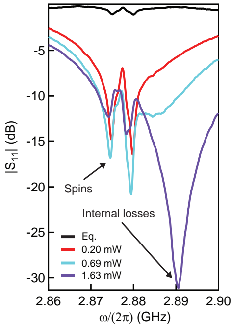
Figure 4.22: Reflected amplitude |S_{11}| under continuous optical irradiation. The absorption of the spins under optical irradiation with 0.2 (red), 0.69 (light blue) and 1.63 mW (blue) is compared to the one at equilibrium (black line). The curves show the |0\rangle \rightarrow |\pm\rangle spectroscopic transitions of the spins, with a spin absorption that increases with P_L because of increasing spin polarization. The additional broad peak at \omega_r that increases with P_L corresponds to the internal losses induced by the optical irradiation.
