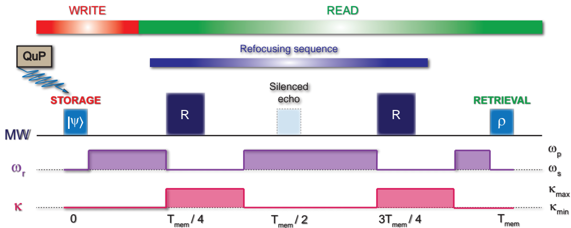
Figure 2.8: Quantum memory protocol. The cavity-field state |\psi\rangle delivered by the QuP is stored at t = 0 and retrieved at t = T_{mem} .
