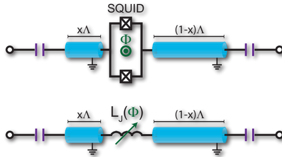
Figure 1.13: The frequency tunable resonator.
