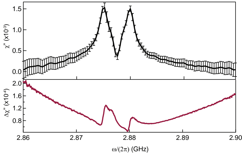
Figure 4.24: Imprecisions on the conversion from |S_{11}| to \chi'' . (top) The spin susceptibility \chi'' under continuous optical irradiation at P_L = 0.2 mW with its error bars and (bottom) the one-standard deviation. The imprecisions increase when getting far from resonance, suggesting that the spin susceptibility is not reliable in the wings.
