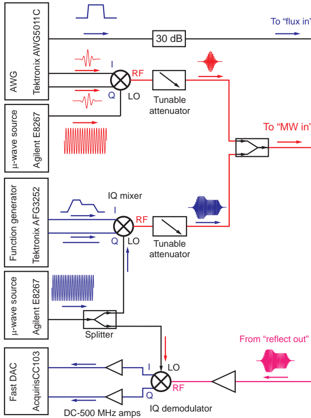
Figure 3.14: Configuration of the setup at room temperature.
