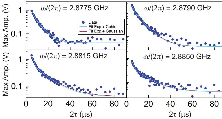
Figure 4.63: Gaussian ( n = 2 ) and cubic ( n = 3 ). Measured (dots) and fitted (red line) echo decay for a selection of probe frequency.
