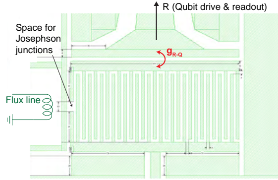
Figure 3.8: The qubit and its coupling to the readout circuitry. Schematic of the simulated chip geometry, showing the Transmon capacitance, the space for the Josephson junction and the coupling to the readout circuitry.
