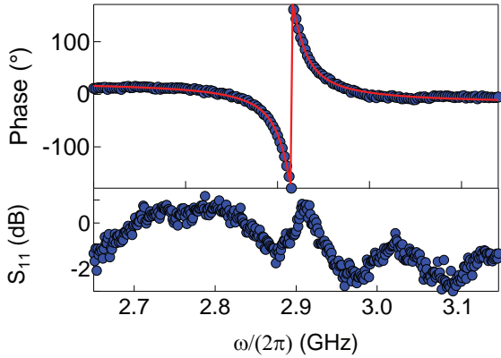
Figure 5.14: Spectrum of the resonator B at f_W . The fit of the phase response (red line) yields resonator frequency \omega_B/2\pi = 2.907 GHz and quality factor Q = 195 \pm 5 . The effect of spurious resonance in the measurement setup is visible in amplitude.
