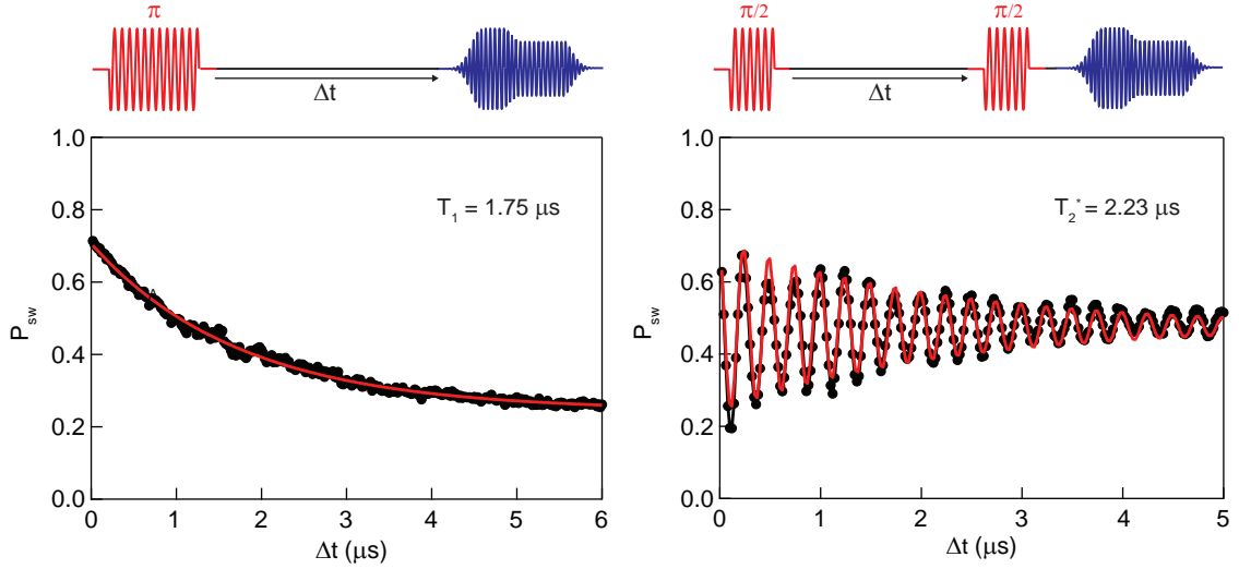
Figure 3.23: Measurement of the qubit coherence times. (left) T_1 measurement. The switching probability P_{sw} is measured as a function of the delay time \Delta t between the preparation of the qubit in the excited state |e\rangle and the actual measurement of the qubit state (black points). The line is a fit by a decaying exponential yielding T_1^Q = 1.75\mu s . (right) T_2^* measurement. The switching probability P_{sw} is measured at the end of the Ramsey sequence as a function of the delay time \Delta t between the two \pi/2 pulses. The line is a fit by an exponentially decaying sine function yielding T_{2,Q}^* = 2.23\mu s .
