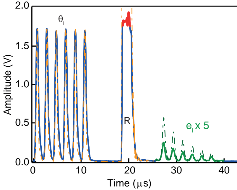
Figure 4.47: Retrieval of multiple weak microwave pulses initially stored in the spin ensemble: the comparison with numerical simulations.
