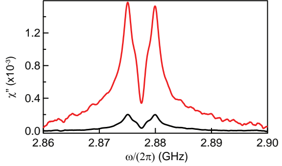
Figure 4.23: Spin susceptibility \chi'' under continuous optical irradiation at P_L = 0.2 mW. The measured reflected amplitude |S_{11}| has been calibrated for the measurement lines ( G(\omega) ), and |r| further converted in spin susceptibility \chi'' . The spin susceptibility under continuous optical irradiation at P_L = 0.2 mW (red) is larger than at equilibrium (black) by a factor 6.7.
