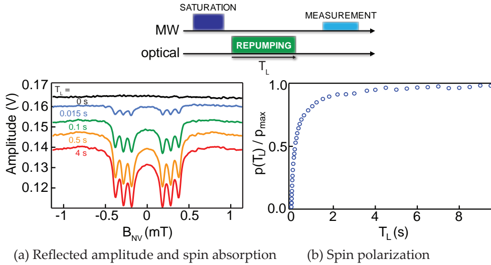
Figure 12: Read experiment: active reset of the spins. (a) Reflected amplitude for 1.5 mW laser power and different duration T_L . The curves show the spectroscopic signatures of the spins, with an amplitude that increases with T_L because of increasing spin polarisation. (b) Relative spin polarisation dependence on T_L .
