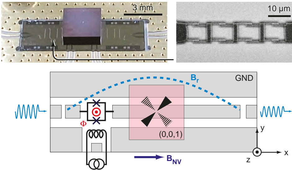
Figure 3.2: Strong coupling of a spin ensemble to a superconducting resonator [19]: scheme of the experiment. (top left) A diamond crystal containing NV center spins is placed on top of the superconducting circuit and positioned in the middle of the superconducting coplanar resonator. (top right) A SQUID array is inserted in the central conductor to tune the resonator frequency with an on-chip wire producing a flux \Phi in the SQUIDs. (bottom) A magnetic field B_{NV} is applied, making the same angle with the four possible NV axis orientations.
