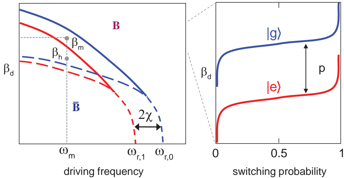
Figure 1.24: Single-shot qubit readout. (a) Same CJBA phase diagram as on Fig. 1.12 for a CJBA embedding a qubit that shifts the diagram by \pm\chi when being in its |g\rangle and |e\rangle states, respectively. (b) Probability of switching from \bar{\mathbf{B}} to \mathbf{B} as a function of the CJBA input drive amplitude \beta_d , shown for an embedded qubit in state |g\rangle (blue) or |e\rangle (red).
