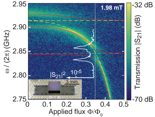
Figure 7: Spectroscopic evidence for spin ensemble-resonator strong coupling [19]. The resonator transmission spectrum shows two avoided level crossings whenever the tunable resonator frequency crosses the NV resonance frequencies.
