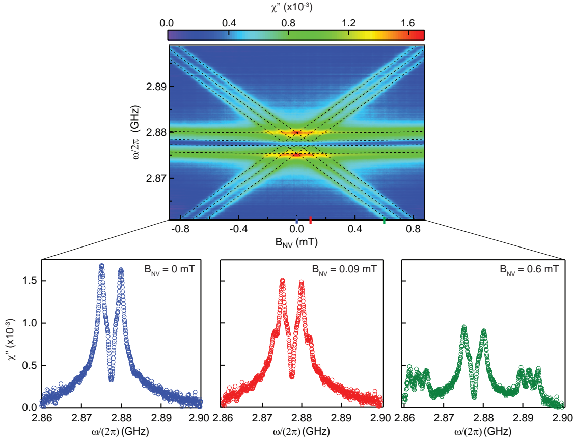
Figure 4.50: Full NV spectroscopy. The spin susceptibility is measured as a function of the magnetic field B_{NV} by microwave reflection measurement. The spin signal is increased by polarizing the spins by a continuous 0.2 mW optical irradiation. Blue, red and green curves are cut at B_{NV} = 0, 0.09, 0.6 mT.
