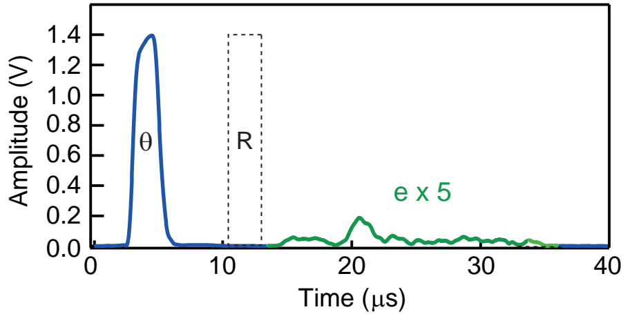
Figure 4.45: Retrieval of a few-photon field initially stored in the spin ensemble. The echo e with \sim 0.02 photons in the resonator is obtained for a \theta pulse populating the resonator with only \sim 100 photons. The refocusing pulse (dashed line) was suppressed in the room-temperature detection chain by a microwave switch to avoid saturating the follow-up amplifiers.
