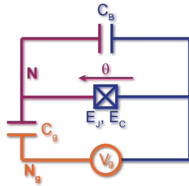
Figure 1.16: Circuit schematic of a Cooper Pair Box. A superconducting island (purple) is connected to a reservoir (blue) through a Josephson junction with Josephson energy E_J , and a capacitance C_J . This island is also electrostatically coupled to ground through a geometric capacitor C_B , and to a voltage source V_g through a capacitor C_g . The gate circuit (yellow) can be used to induce an offset charge on the island.
