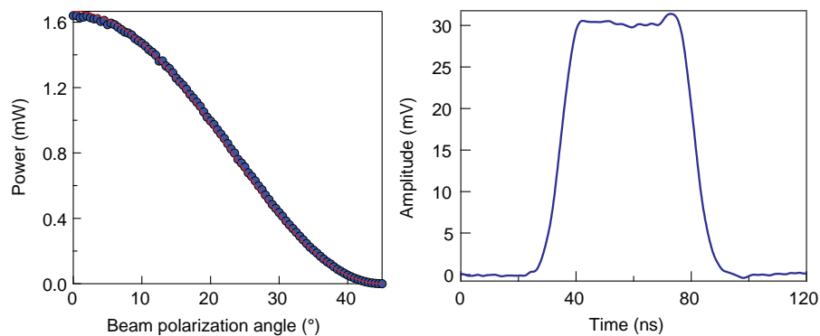
Figure 4.12: Optical pulses. (left) The optical power at the sample stage is controlled with 10 \mu\text{W} resolution up to 1.65 mW using a half wave plate mounted on a motorized rotation stage. (right) The optical pulse shape is designed with 10 ns resolution by double pass in the AOM.
