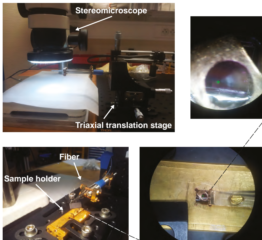
Figure 4.14: Alignment setup. (top left) The fiber is mounted on a triaxial translation stage, placed under a stereomicroscope with large working distance and dropped through a hole in the sample box (bottom left) to be attached to the sample (bottom right). The top right picture shows the light beam reflected on the niobium (green spot) and the inductance (black square) as seen through the optical microscope during the alignment process.
