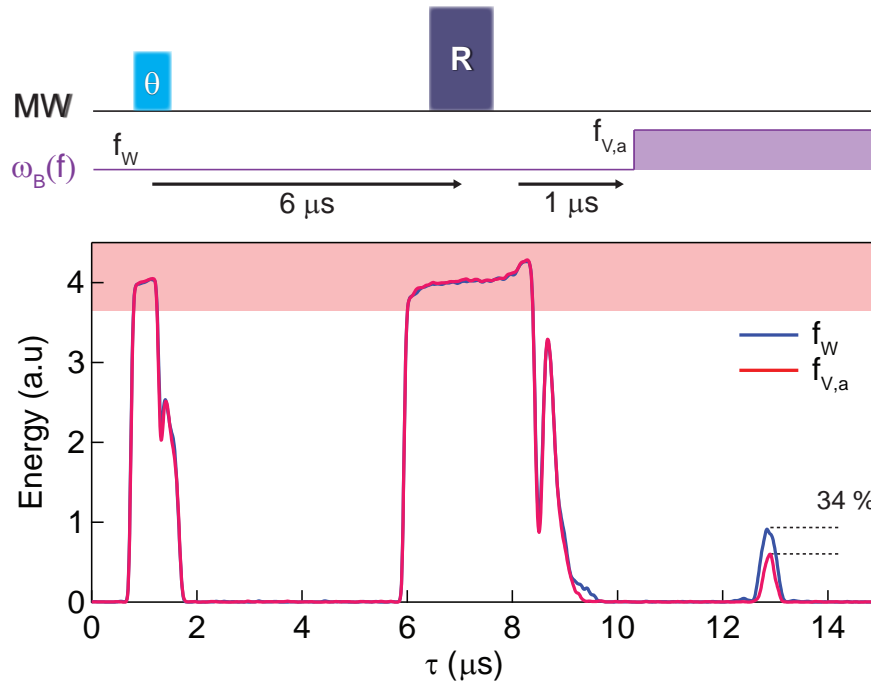
Figure 5.18: Partial silencing of the echo by dynamical detuning of the resonator. (top) Protocol. The Hahn echo sequence at f = f_W of Fig. 5.16 is applied, followed 1 \mu\text{s} after the application of the refocusing pulse by a detuning of the cavity at \omega_B(f_{V,a}) . The sequence is repeated without detuning for comparison. (bottom) Measured reflected amplitude with (red) and without (blue) detuning after the refocusing pulse. The echo obtained when the resonator is at \omega_B(f_{V,a}) is reduced by 34 % in energy.
