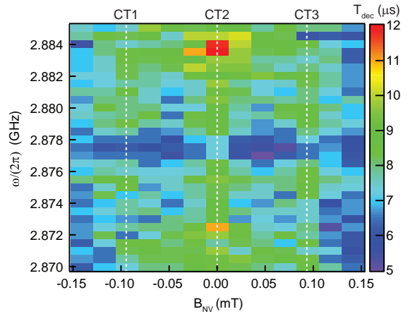
Figure 4.54: Two-dimensional plot of the characteristic decay time T_{\text{dec}}(\omega, B_{\text{NV}}) . At B_{\text{NV}} = B_{\text{CT1}}, B_{\text{CT2}}, B_{\text{CT3}} , the measured characteristic decay time is long independently of the probe frequency, confirming the absence of spurious effect.
