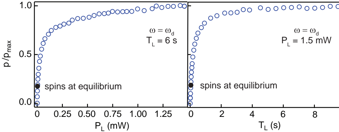
Figure 4.31: Spin reset efficiency p/p_{\text{max}} . (left) The relative spin polarization for T_L = 6 \text{ s} as a function of P_L increases then saturates. This corresponds to our observation in Section IV.4.2, suggesting that the maximum polarization accessible by optical repumping is reached. (right) The relative spin polarization for P_L = 1.47 \text{ mW} as a function of T_L increases then saturates. Since P_L > P_{L,\text{max}} , the saturation corresponds to the maximum polarization accessible by optical repumping.
