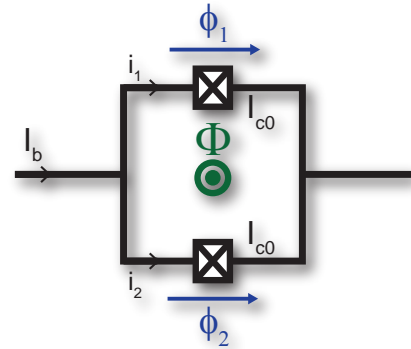
Figure 1.10: Electrical scheme of a SQUID.
