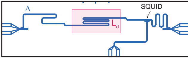
Figure 3.9: The bus resonator: the design. It is made with a section of CPW transmission line terminated at both ends with elbow couplers. A SQUID is embedded in its central conductor to make its frequency tunable. The diamond covers a length L_d of the resonator length \Lambda .
