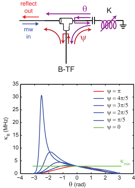
Figure 5.21: Schematic of the circuit and simulations. The microwave tee can be either a commercial tee connected to the circuit K and B -TF (placed in separated sample box) via microwave cables, or patterned directly together with K and B -TF on a single circuit. The simulations of this circuit relies on the formulas in [125].
