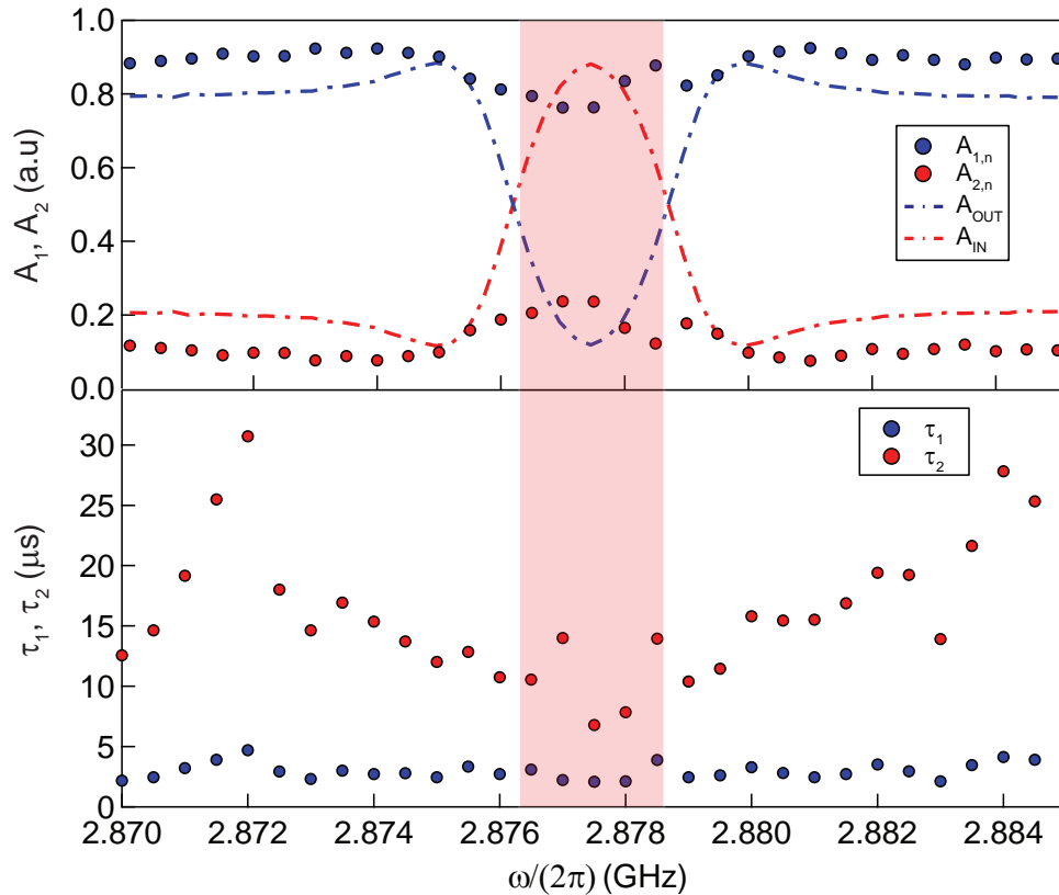
Figure 4.61: Comparison of the double exponential weights to the theory. The red area corresponds to the region in which the fit are irrelevant.
