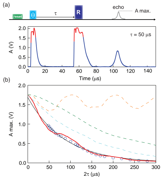
FIG. 3. (a) Hahn echo sequence. The spins are first reset in their ground state by a laser pulse of power 280 \mu\text{W} and duration 0.2 s. A first 1 \mu\text{s} microwave pulse \theta at \omega_r , of power -71 dBm, induces a transverse magnetization which decays within T_2^* . A 1 \mu\text{s} -long microwave refocusing pulse ( R ) of power -20 dBm is applied at \tau = 50 \mu\text{s} , which rephases the spins at 2\tau . The microwave amplitude (blue curve) shows both the reflection of the two microwave pulses driving the spins (with their amplitude trimmed by saturation of our detection chain, as indicated in red), as well as the echo emitted at 2\tau upon rephasing of the spins. (b) Measured decay of the echo amplitude A as a function of 2\tau (open circles). Calculated decay due to a bath of 213 ppm of ^{13}\text{C} (dashed orange curve), 0.6 ppm of P1 centers causing spectral diffusion (dashed green line), 0.2 ppm of NV centers causing instantaneous diffusion (dashed blue line), and the combination of the three contributions (solid red line). The theory curves have been scaled in amplitude according to the data. An exponential fit (black solid line) yields a coherence time T_2 = 84 \mu\text{s} .
