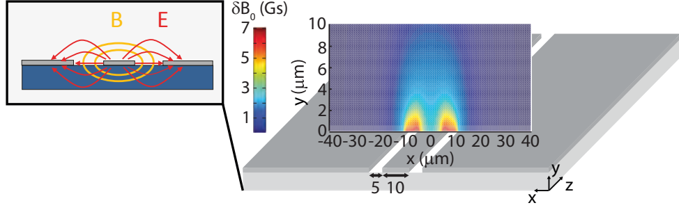
(a) The electromagnetic field of a CPW resonator
