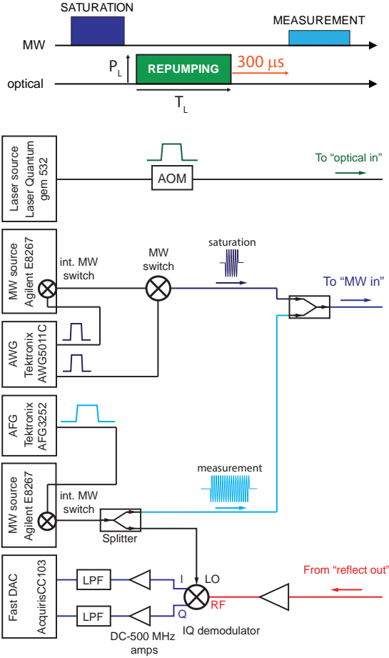
Figure 4.27: Protocol and setup for active spin polarization measurement.
