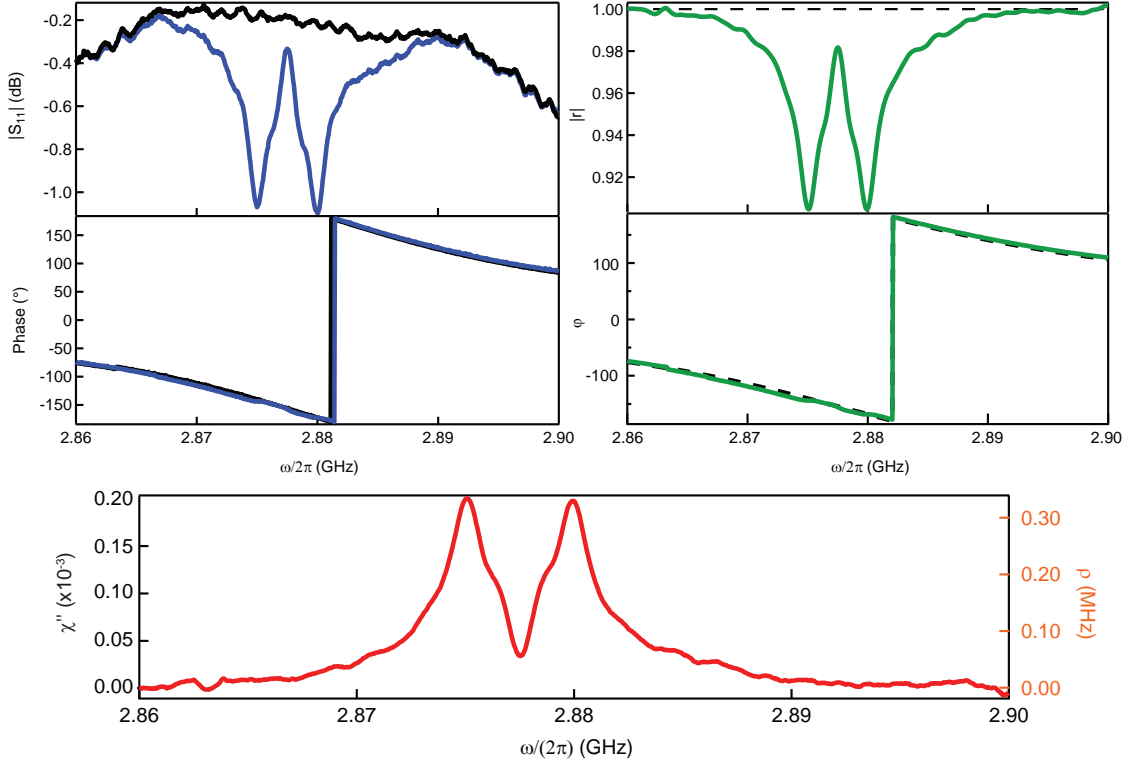
Figure 4.16: Response of the spins at zero magnetic field as seen through the resonator. (top left) Amplitude and phase of the reflection coefficient S_{11} showing the resonator resonance on the phase and the spin absorption on the amplitude. (top right panel) Corresponding calibrated reflection coefficient. (bottom) Measured spin signal expressed in spin susceptibility \chi'' (on the left vertical axis) and in coupling density profile (on the right vertical axis).
