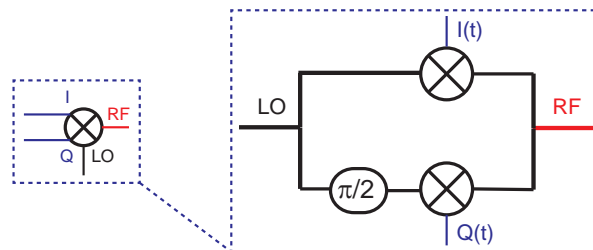
Figure 3.17: Diagram of an IQ mixer.
