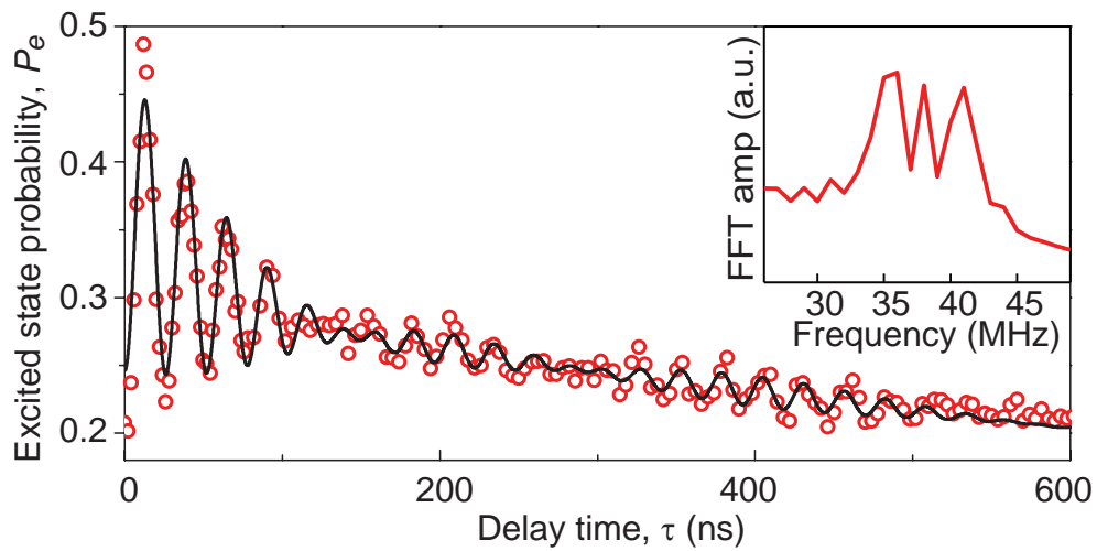
Figure 3.39: Ramsey-like experiment on the spin ensemble at the single-photon level. Measured (red circles) and calculated (black line) probability P_e(\tau) , as well as its Fourier transform (inset) revealing the NV centers hyperfine structure.
