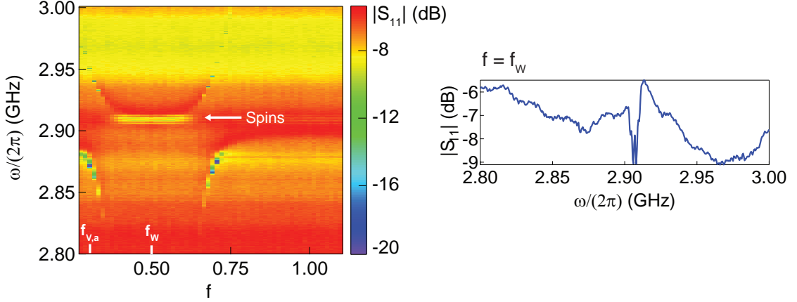
Figure 5.15: Reflection spectrum |S_{11}| at B_{NV} = 1.26 mT. The spin absorption is visible on the reflected amplitude at \omega_B/2\pi = 2.907 GHz. At f = f_W , the spins are on resonance with the resonator and refocusing pulse can be applied. At f = f_{V,a} , the spins are out of resonance.
