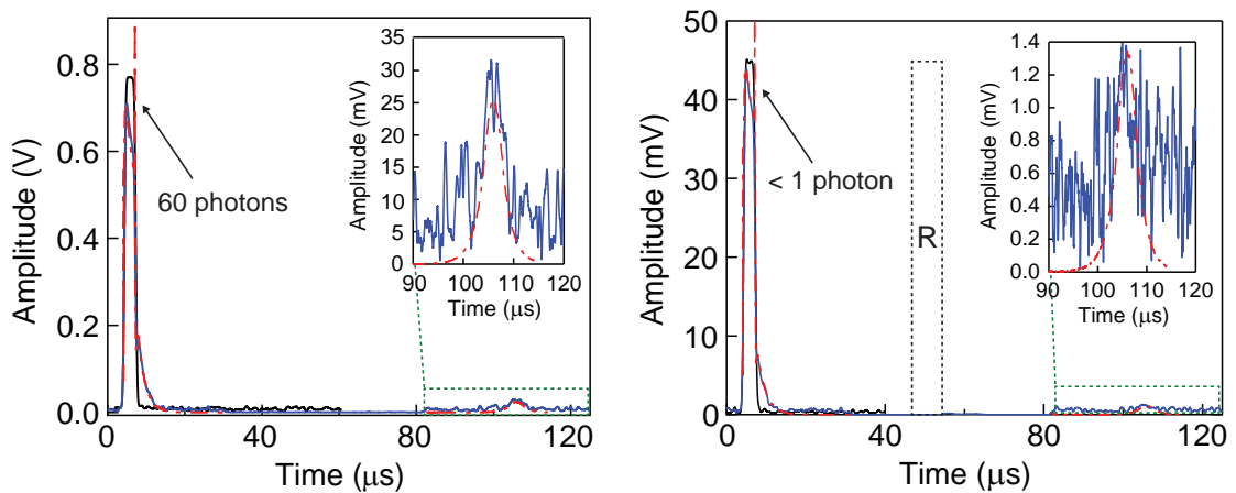
Figure 5.6: Retrieval of few-photon fields initially stored in the spin ensemble with 0.3 % efficiency after 100 \mu\text{s} . The echo e is obtained for a low power incoming \theta pulse populating the resonator with only \sim 60 photons (left) and < 1 photon (right). The refocusing pulse was suppressed in the room-temperature detection chain by a microwave switch to avoid saturating the follow-up amplifiers. The results of numerical simulations performed by Brian Julsgaard are superimposed on the graphs (dash-dotted red lines).
