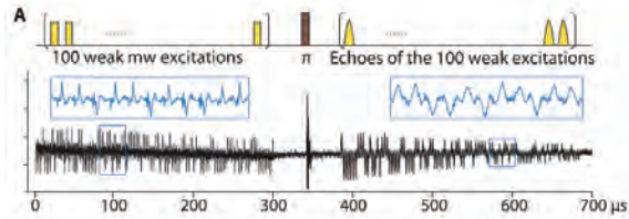
Figure 4.2: Storage of Multiple Coherent Microwave Excitations in an Electron Spin Ensemble [102]. Storage of 100 microwave excitations. After the refocusing pulse the stored excitations are recovered in reverse time order.
