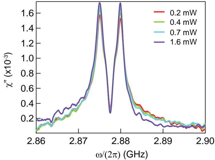
Figure 4.25: Dependence of the spin susceptibility on the optical power \chi''(P_L) . The shape of the spin susceptibility is unchanged but its amplitude increases with the optical power P_L suggesting an increasing spin polarization. The slight asymmetry which appears at high optical power is attributed to the imprecisions on the conversion from |S_{11}| to \chi'' , that increases with the optical power.
