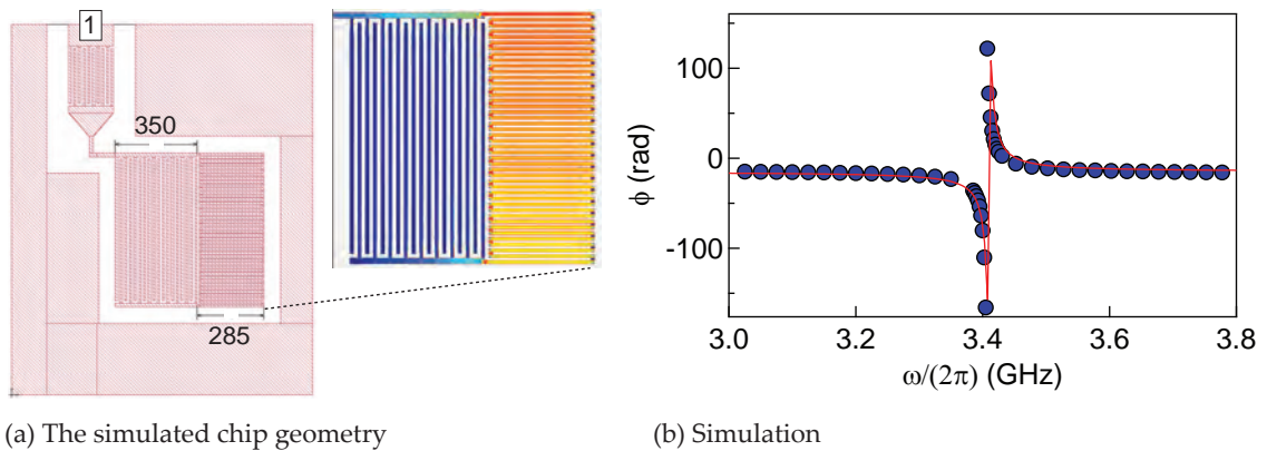
Figure 1.6: Implementation of a superconducting resonator with lumped electrical elements. (a) Schematic of the simulated chip geometry, showing the resonator and the coupling capacitance to an input port with impedance 50 \Omega . The computed alternative current flowing in the inductance is shown in the inset. (b) Computed (dots) and fitted (lines) reflected phase \phi , yielding \omega_r/(2\pi) = 3.41 \text{ GHz} and Q = 300 .
