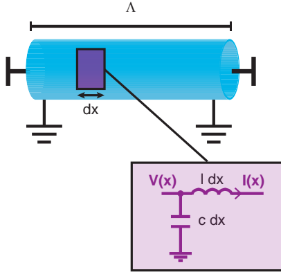
Figure 1.7: Distributed-element resonators. A transmission line, with open circuits at each end, constitutes a microwave resonator.
