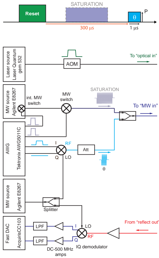
Figure 4.33: Protocol and setup for response of the spins measurement.
