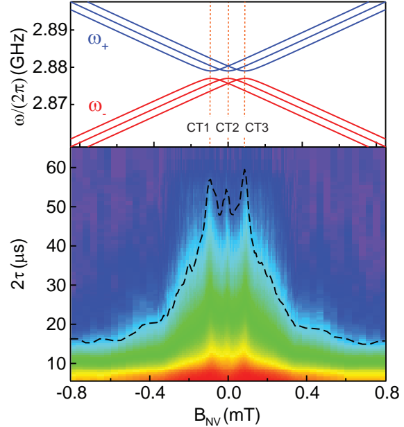
Figure 14: Decay of the spin-echo amplitude as a function of the external magnetic field. The coherence time is enhanced at the three clock transitions.
