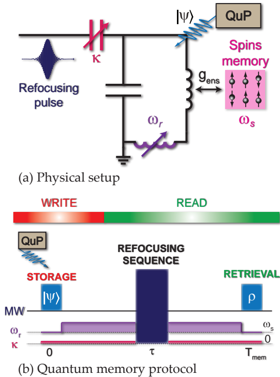
Figure 3: Spin ensemble quantum memory principle. (a) Quantum memory circuit. The resonator, with frequency \omega_r and damping rate \kappa tunable at the nanosecond scale, is coupled to the spin ensemble (frequency \omega_s ) with coupling strength g_{\text{ens}} . An external processor (QuP) delivers a quantum state |\psi\rangle to the bus resonator, to be stored into the spin-based memory. Refocusing pulses are applied to the spins via the resonator. (b) Schematic timing of pulses and cavity parameters \omega_r and \kappa . The quantum state delivered by QuP is stored in the spin ensemble (write operation). A refocusing sequence acts as time-reversal for the spins and triggers the retrieval of the stored quantum state as an echo (read operation).
