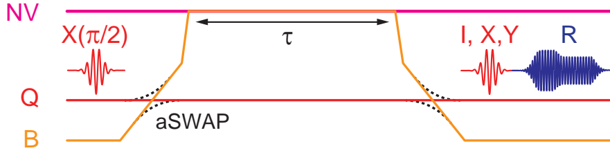
Figure 3.36: Protocol for storage a coherent superposition of states from the qubit to the spin ensemble. The sequence shows the microwave pulses used for exciting the qubit in \frac{1}{\sqrt{2}}(|g\rangle + |e\rangle) (red) and for reading it out (blue), as well as transition frequencies of the quantum bus (orange), qubit (red), and spins (magenta). Quantum state tomography is performed to determine the qubit state by applying either I, X, or -Y operation to the qubit before reading out the Z component.
