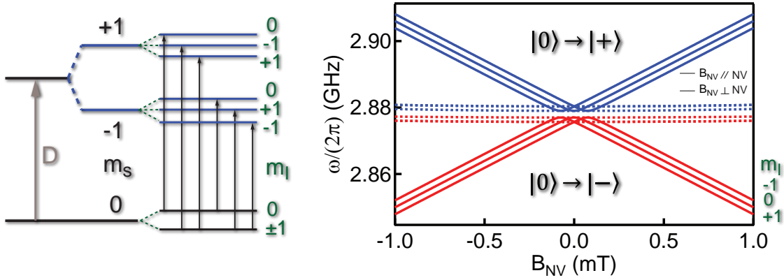
Figure 1.29: NV energy diagram showing the Zeeman and hyperfine structure of the electronic ground state under a magnetic field applied parallel (perpendicular) to the NV center axis. Six microwave transitions are allowed. Under magnetic field applied perpendicular to the NV axis, the transitions |m_S = 0, m_I = \pm 1\rangle \rightarrow |m_S = +1, m_I = +1\rangle and |m_S = 0, m_I = \pm 1\rangle \rightarrow |m_S = +1, m_I = -1\rangle (respectively |m_S = 0, m_I = \pm 1\rangle \rightarrow |m_S = -1, m_I = +1\rangle and |m_S = 0, m_I = \pm 1\rangle \rightarrow |m_S = -1, m_I = -1\rangle ) are degenerated.
