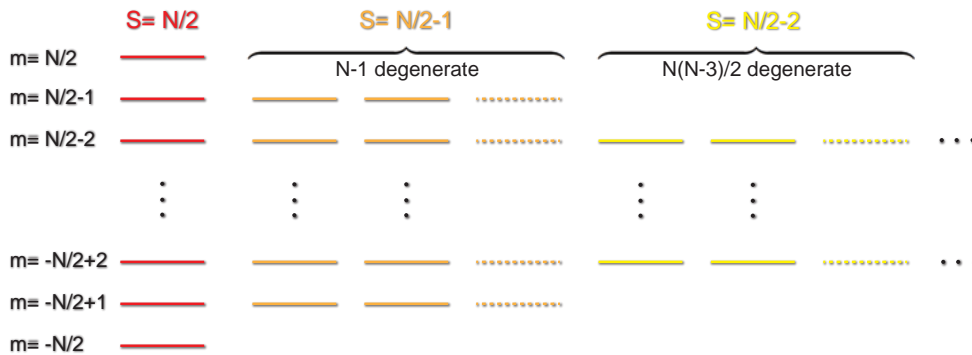
Figure 1.34: Energy level diagram of an ensemble of N spins-1/2. States \mathcal{S} \neq N/2 are highly degenerate. There is one ground state corresponding to |N/2, -N/2\rangle , N states with a single excitation m = -N/2 + 1 , among which 1 state |N/2, -N/2 + 1\rangle and (N - 1) of the form |N/2 - 1, -N/2 + 1\rangle .
