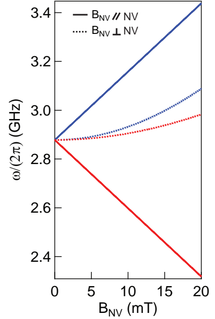
Figure 1.28: Energy states dependence of the microwave transitions \omega_{\pm} under a magnetic field, applied parallel (perpendicular) to the NV center axis showing a linear (quadratic) Zeeman effect.
