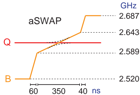
Figure 3.29: The aSWAP.
