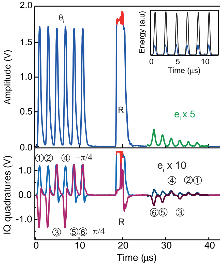
Figure 4.43: Retrieval of multiple weak microwave pulses initially stored in the spin ensemble. (top) Amplitude of the measured output signal showing the reflected pulses \theta_i (after partial absorption by the spins) and R (its amplitude being trimmed by amplifier saturation, shown in red), as well as the six re-emitted echoes e_i (magnified by a factor 5). inset: The comparison between the energies of the reflected \theta_i pulses with the spins saturated (black line) or reset in their ground state (blue line) shows that about 75% of the incident power is absorbed by the spins. (bottom) IQ quadratures of the output signal, showing that the e_i pulses (magnified by 10) are recovered with phase -(\varphi_i - \varphi_r) , as expected.
