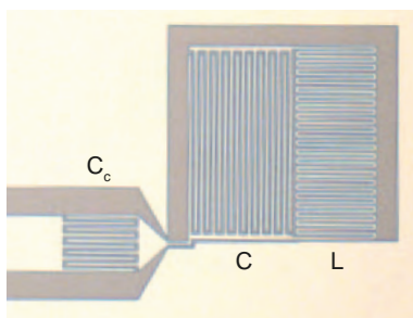
Figure 1.5: Picture of a lumped-element resonator.
