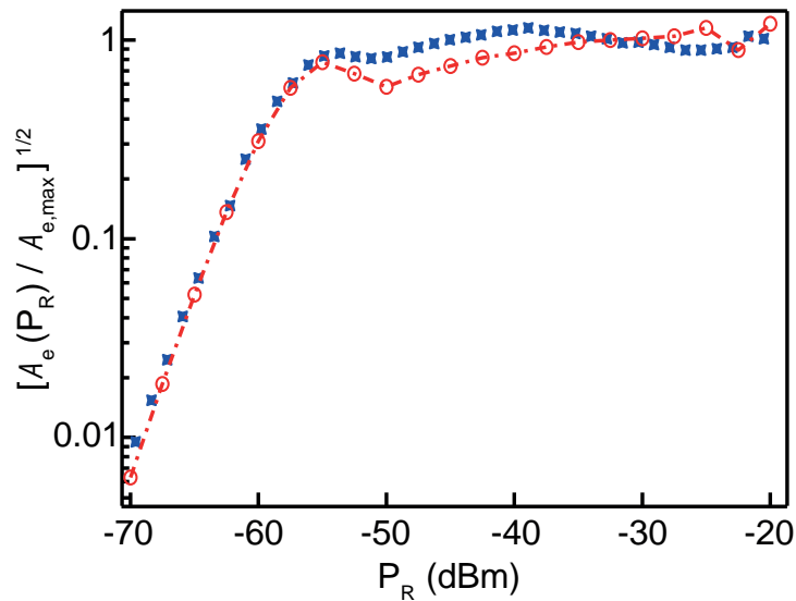
Figure 4.41: Dependence of the echo amplitude on the refocusing pulse power. Experimental (crosses) and simulated and rescaled (open circles) area of the echo as a function of the refocusing pulse power P_R .
