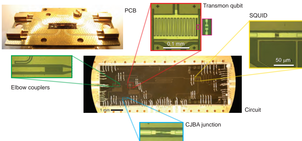
Figure 3.11: The fabricated circuit with panels zooming to its most important features.
