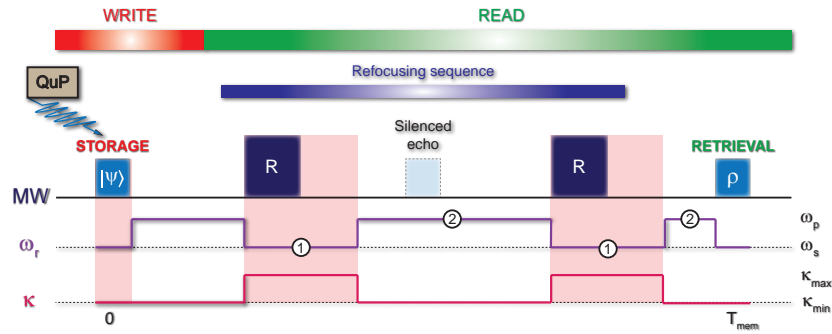
Figure 5.9: Dynamical tuning of the resonator along the memory protocol. The periods of resonance with the spins are marked in red. In 1, the resonator is on resonance with the spins and contains a large intracavity field due to the applications of the refocusing pulses. In 2, the resonator is detuned and contains low intracavity field.
