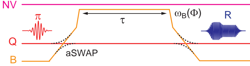
Figure 3.32: Protocol for storage of a single quantum of excitation from the qubit to the spin ensemble. The sequence shows the microwave pulses used for exciting the qubit in |e\rangle (red) and for reading it out (blue), as well as transition frequencies of the quantum bus (orange), qubit (red), and spins (magenta).
