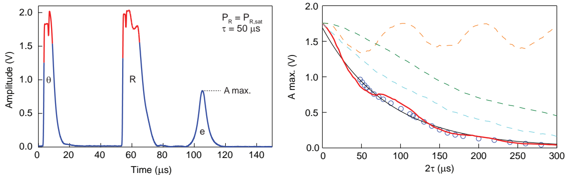
Figure 5.5: Hahn echo sequences and spin coherence times. (left) The echo (e) is observed at time 2\tau = 100\ \mu\text{s} . Saturation of the amplifiers (shown in red) limits the measurable amplitude to about 1.5 V. (right) Measured (dots) and calculated (red solid line) decays of the echo maximum amplitude as a function of \tau . The calculated decay is a combination of the decays due to the bath of 213 ppm of ^{13}\text{C} (dashed orange curve), 0.6 ppm of P_1 centers causing spectral diffusion (dashed green line) and 0.2 ppm of NV centers causing instantaneous diffusion (dashed blue line). An exponential fit (black solid line) yields a coherence time T_2 = 84\ \mu\text{s} .
