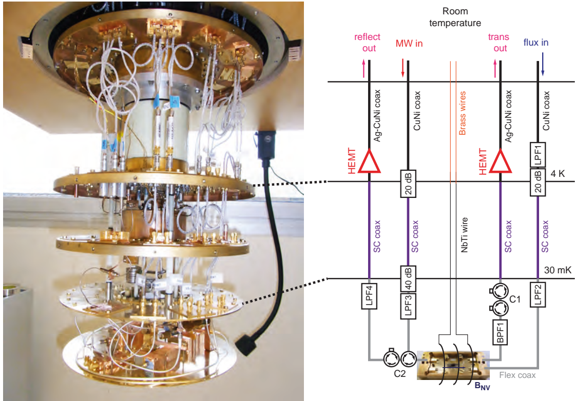
Figure 3.13: Picture and wiring scheme of the dilution refrigerator. LPF 1 , LPF 2 , LPF 3 , and LPF 4 are low-pass filters with cutoff frequencies 1.35 GHz, 450 MHz, 5.4 GHz, and 5.4 GHz, respectively. BPF 1 is a band-pass filter with a bandwidth of 2.5 - 4 GHz. C 1 , C 2 are double circulator. CuNi coax is a coaxial cable made of CuNi, and Ag-CuNi coax is a silver-plated CuNi coaxial cable. SC coax is a superconducting NbTi coaxial cable. Flex coax is a low-loss flexible coaxial cable. Rectangles represent ports terminated by 50 \Omega . The cryogenic microwave amplifier is a CITCRYO 1-12 from Caltech, with gain \sim 38 dB and noise temperature \sim 5 K at 3 GHz. A DC magnetic field B_{NV} is applied parallel to the chip by passing a DC current through an outer superconducting coil. The sample box and the coil are surrounded by two magnetic shieldings consisting of a lead cylinder around which permalloy tape is wrapped. The sample box, coil, and the shieldings are thermally anchored at the mixing chamber.
