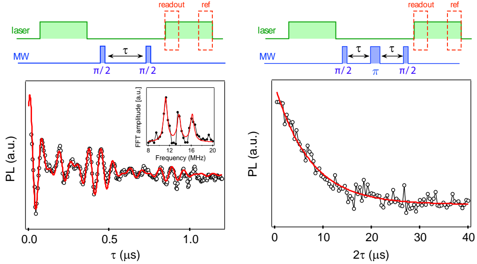
Figure 3.7: The diamond: coherence times at room temperature. (left) Ramsey fringes recorded for the subset of [111]-oriented NV centers with a microwave detuning \delta = 13 MHz from the ESR line at \omega_{+1}/2\pi = 2.915 GHz. The laser pulses used in the Ramsey sequence have a duration of 30 \mu\text{s} and the laser power is set at 40 mW. For data analysis, the NV center PL recorded during the first 10 \mu\text{s} of the laser pulses is used for spin-state read-out while the PL recorded during the last 10 \mu\text{s} is used as reference. The red solid line is data fitting with the function \exp[-\tau/T_2^*] \times \sum_{i=-1}^1 \cos [2\pi(\delta + iA_{\parallel})\tau] . The inset shows the Fourier-transform of the free induction decay. Solid lines are data fitting with Lorentzian functions. (right) Measurement of the coherence time T_2 for the subset of [111]-oriented NV centers using a \pi/2 - \tau - \pi - \tau - \pi/2 spin echo sequence. Data fitting with an exponential decay leads to T_2 = 7.3 \pm 0.4 \mu\text{s} .
