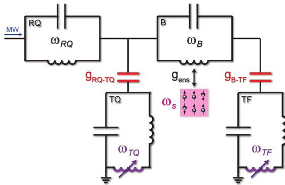
Figure 5.20: Schematic of the circuit. The circuit B-TF is coupled to the external measurement lines via a resonator RQ, that can be detuned dynamically.
