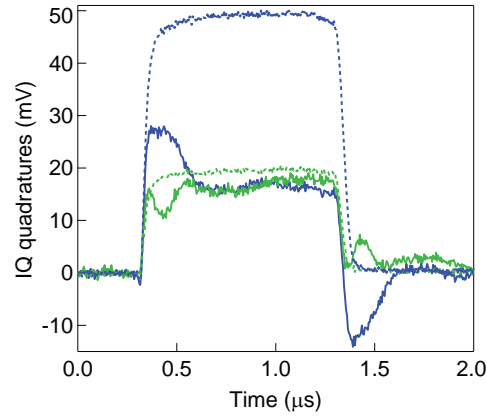
Figure 4.34: Response of the spins to an incoming weak microwave pulse. In-phase quadrature (blue) and out-of-phase (green) quadratures of the reflected field for an applied square microwave pulse of power P_0 = -90 dBm. The dashed lines correspond to the same measurement with the spins saturated.
