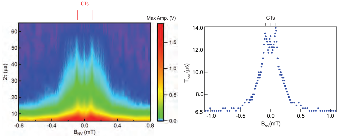
Figure 4.53: Dependence of the echo decay on the magnetic field B_{\text{NV}} . (left) Two-dimensional plot of the echo amplitude A(B_{\text{NV}}, \tau) . The spins of the N-Orth group contribute induce longer decay tails at the three magnetic field values B_{\text{NV}} = -0.09, 0, +0.09 mT corresponding to the clock transitions. The overall effect in the zero-field region arises from the m_I = 0 spins of the N-Orth group contribution. (right) Corresponding time T_{\text{dec}} at which the amplitude of the echo is reduced by 10. At the CTs, the characteristic decay time T_{\text{dec}} shows an enhancement by a factor \sim 2 .
