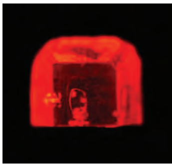
Figure 5.1: The diamond sample. The picture of the diamond is taken under continuous irradiation at 532 nm. The red color corresponds to the photoluminescence of the NVs. An inclusion is visible on the top face.
