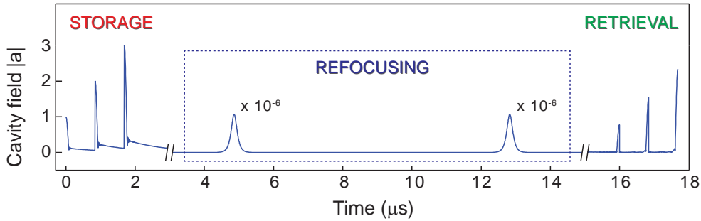
Figure 5: Results of numerical simulations , showing that successive cavity field states can be stored and retrieved with 80 % efficiency with our memory protocol.
