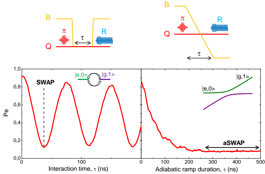
Figure 3.28: Comparison between resonant and adiabatic SWAP pulses. (left) principle of a resonant SWAP. After excitation of the qubit in |e\rangle , B is put suddenly into resonance with Q for an interaction time \tau during which |e,0_B\rangle and |g,1_B\rangle swap periodically. After a time \tau = 37 ns, the qubit excitation is transferred to B. (right) principle of an adiabatic SWAP (aSWAP). The qubit is excited in |e\rangle , after what \omega_B is ramped through \omega_Q in a time \tau , and the state of Q is finally read-out. For long enough ramp durations (for this sequence \tau > 300 ns), the qubit excited state population is fully transferred into the bus.
