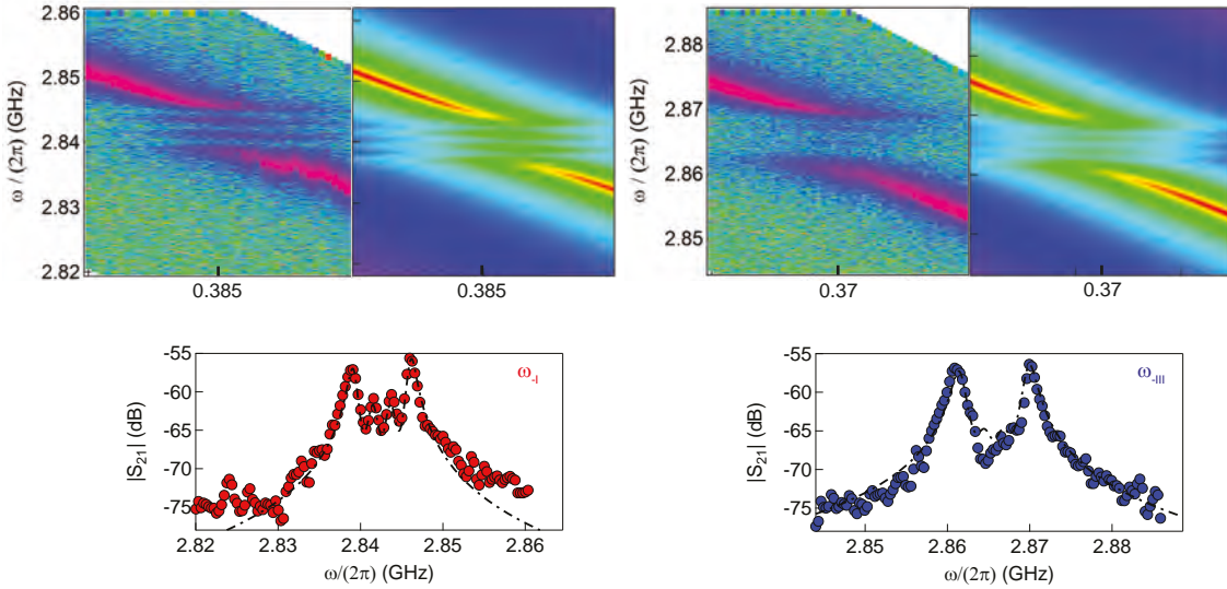
Figure 3.31: Comparison to the model. (top) Measured and computed spectrum around the |0\rangle \rightarrow |- \rangle transition of the spin group I (left) and III (right). Color scale goes from -70 dB to -40 dB. (bottom) Measured (dots) and computed (line) transmission spectrum close to the middle of the anticrossing with the |0\rangle \rightarrow |- \rangle transition of the spin group I (left) and III (right). The asymmetries that results from a slight detuning between the spin central frequency and the resonator is well explained by the model.
