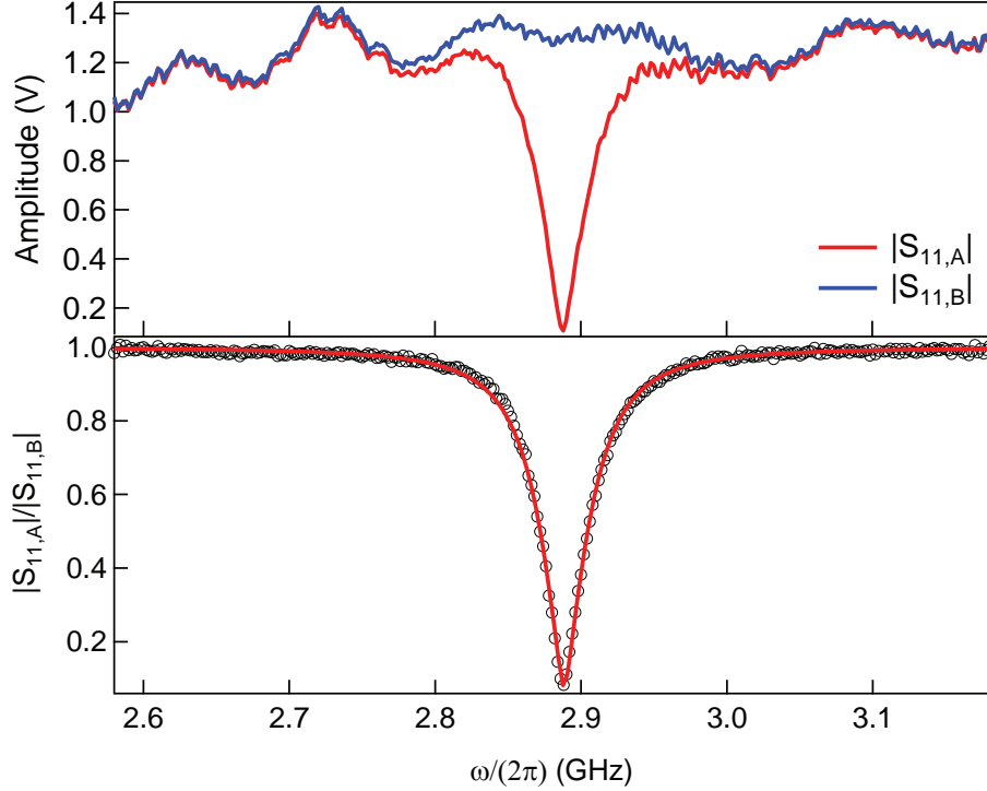
Figure 4.20: Reflected amplitude |r| under optical irradiation at P_L = 1.6 mW, with the spins saturated. (top) The resonator spectrum is probed under laser irradiation ON (red) and OFF (blue). Under laser irradiation, the reflected amplitude reaches almost 0 indicating that the internal losses \kappa_L are on the same order than the external damping rate \kappa (see Section I.1.1.2). The additional internal losses are attributed to the effect of the optical irradiation on the resonator. (bottom) Measured (dots) and fit (red line) of the corresponding calibrated reflected amplitude. The fit with Eq. 4.10 yields \omega_{c,las}/2\pi = 2.888 GHz, \kappa_{las} = 191.6 \pm 1.2 \cdot 10^6 s ^{-1} and \kappa_{L,las} = 164 \pm 1.9 \cdot 10^6 s ^{-1} .
