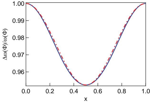
Figure 1.14: Dependence of resonance frequency on the position of the SQUID in the resonator. \Delta\omega_r(x\Lambda, \Phi_f) is shown at fixed applied magnetic flux \Phi_f as a function of x . The line is fitted with Eq. 1.42 (dashed and dotted line)
