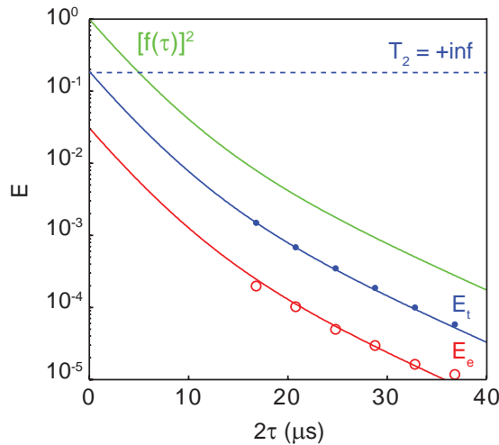
Figure 4.46: The retrieval efficiency. The field recovery efficiency of the experimental (red) and simulated (blue) echo pulses versus the delay 2\tau . The function [f(\tau)]^2 (green) is scaled such that f(\tau = 0) = 1 and shown for comparison. The experimental and simulated retrieval efficiencies follow the function [f(\tau)]^2 as E_e = 0.03|f(\tau)|^2 and E_t = 0.21|f(\tau)|^2 , respectively. The dash-dotted line corresponds to the retrieval efficiency with infinite T_2 .
