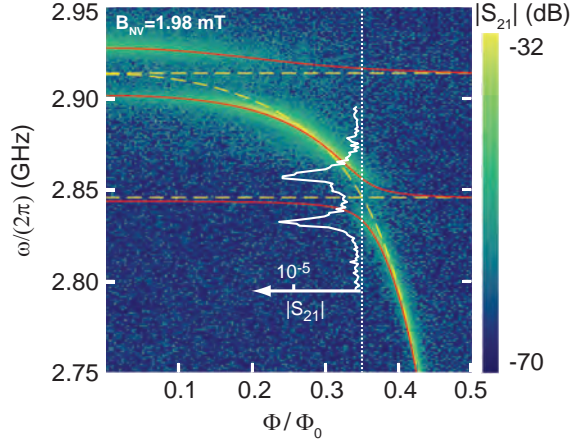
Figure 3.3: Strong coupling of a spin ensemble to a superconducting resonator [19]: spectroscopic evidence for strong coupling. The resonator transmission spectrum S_{21} shows two anticrossings whenever the tunable resonator frequency crosses the NV transitions |0\rangle \rightarrow |+\rangle and |0\rangle \rightarrow |-\rangle . Red solid (yellow dashed) lines are fits to the eigenfrequencies of the coupled (decoupled) resonator-spin system as described in Section I.3.2.1. A transmission spectrum (white overlay) is also shown in linear units in the middle of the anticrossing with the NV transition |0\rangle \rightarrow |-\rangle .
