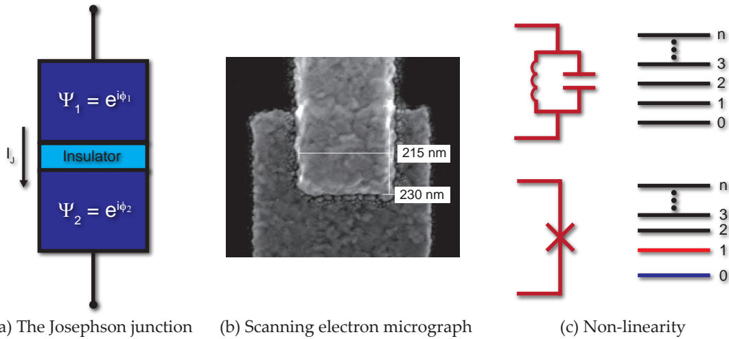
Figure 1.9: The Josephson junction, a non-linear electrical element. (a) A Josephson junction is composed of two superconducting electrodes connected through an insulating barrier. (b) Scanning electron micrograph of a Josephson junction used in this thesis work: the electrodes are made of aluminum and the insulator of aluminum oxide. (c) A LC resonator has equally spaced energy levels which prevents any individual transition from being selectively addressed. A Josephson junction (represented by the X symbol) has unequally spaced energy levels, a property that can be used to bring non-linearity to a circuit.
