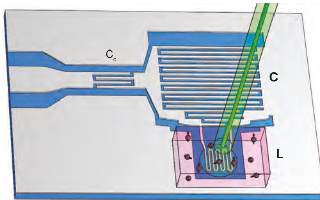
Figure 4.3: Designing the read experiment: schematic of the hybrid circuit. The ensemble of NV center spins (pink) is coupled to a planar superconducting lumped element resonator. Laser pulses can be shone on the diamond through an optical fiber glued to its top face.
