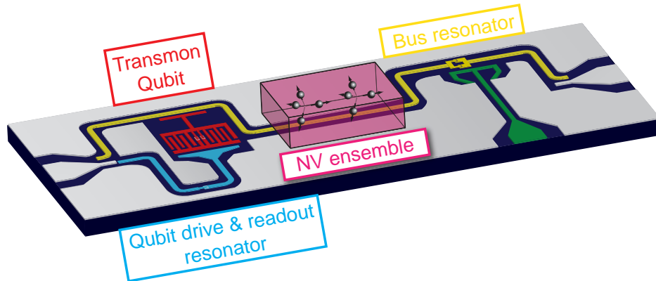
Figure 8: Write experiment: schematic of the hybrid quantum circuit . A transmon qubit (red) is coupled to an ensemble of NV centers electron spins (pink) via a frequency tunable bus resonator (yellow).
