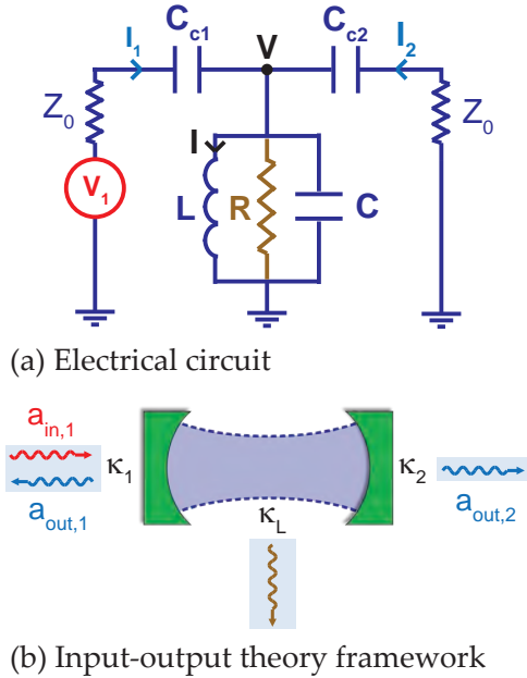
Figure 1.3: Circuit and its equivalent in the input-output theory framework.
