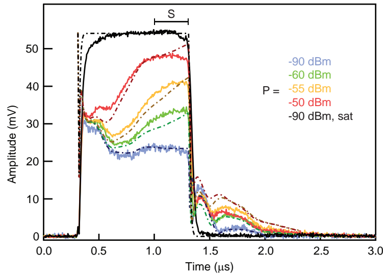
Figure 4.36: Response of the spins to an incoming square pulse. Amplitude of the reflected field for P = -90, -60, -55, and -50 dBm. The curves have been rescaled by \sqrt{P/P_0} for easier comparison, with P_0 = -90 dBm. The pulse extends from 0.3 \mu\text{s} to 1.3 \mu\text{s} , followed in the non-saturated case by the free induction decay signal of the spins. S denoted the steady state region. Dash-dotted lines are simulations (see text).
