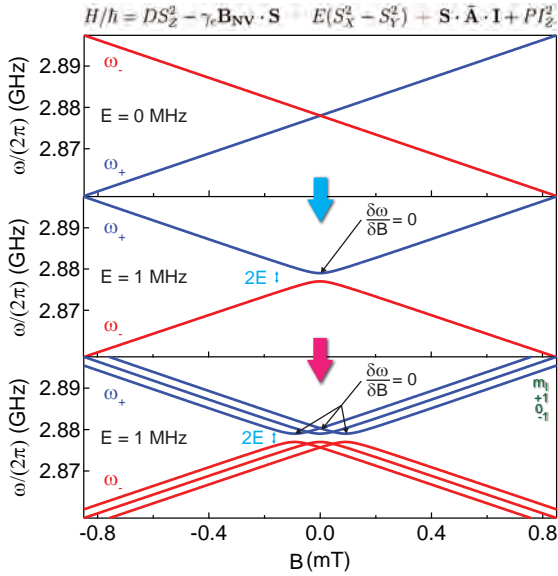
Figure 4.48: Origin. The NV eigenstates present sweet spots d\omega_{NV}/dB = 0 , at which the NV energy is insensitive to first order magnetic field fluctuations. These points originate from an effect of strain and are m_I -dependent.
