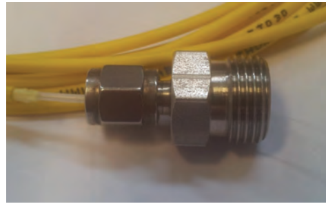
Figure 4.13: The vacuum optical fiber feedthrough. The fiber is crushed into a little piece of Teflon mounted on a Swagelok to enter into the outer vacuum chamber of the dilution refrigerator.
