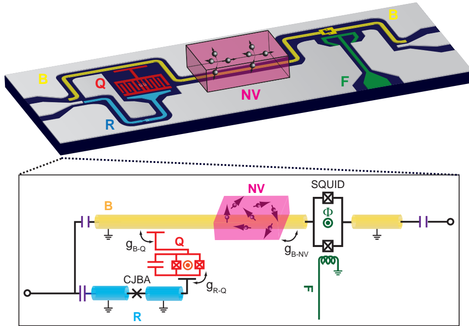
Figure 3.5: Designing the write experiment: schematic of the hybrid quantum circuit. The quantum bus B (in yellow), a coplanar waveguide resonator, is coupled to Q (in red) and to NV (in pink). It contains a SQUID that makes its frequency tunable by applying in its loop a flux via an on-chip current line F (in green). The qubit Q is electrostatically coupled to a nonlinear resonator R (in blue) which is used to manipulate and readout its state.
