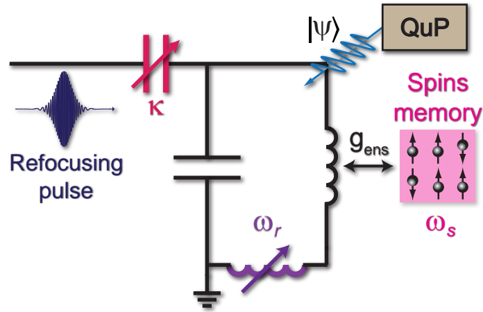
Figure 2.2: Quantum memory circuit. The resonator, with frequency \omega_r and damping rate \kappa tunable at the nanosecond scale, is coupled to the spin ensemble (frequency \omega_s ) with coupling strength g_{\text{ens}} . An external processor (QuP) delivers a quantum state |\psi\rangle to the bus resonator, to be stored into the spin ensemble. Refocusing pulses are applied to the spins via the resonator.
