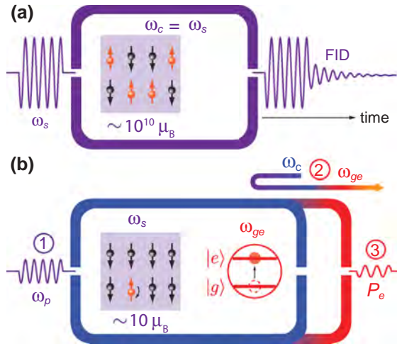
FIG. 1. (Color online) Comparison between conventional pulsed electron spin resonance (ESR) and qubit-detected ESR. (a) Conventional ESR: A spin ensemble is placed in a cavity with a frequency \omega_c and driven with a microwave pulse resonant with the cavity. When the ESR frequency \omega_s matches \omega_c , the spins absorb the microwave pulse, and emit immediately after a free-induction decay (FID) signal into the waveguide connected to the cavity. (b) Qubit-detected ESR: The cavity is now frequency tunable and embeds both the spin ensemble and a superconducting qubit with a frequency \omega_{ge} . In a first step (1), the spins are probed by a spectroscopy pulse with a frequency \omega_p , which excites them if its frequency matches \omega_s . In a second step (2), the cavity frequency is tuned to \omega_c = \omega_s , receives the FID signal from the spins, and is afterwards tuned to transfer this signal to the superconducting qubit at \omega_{ge} . Finally (3) the qubit excited state probability P_e(\omega_p) is measured, mapping the spins absorption spectrum. Very low excitation powers can be used given the high sensitivity of the method.
