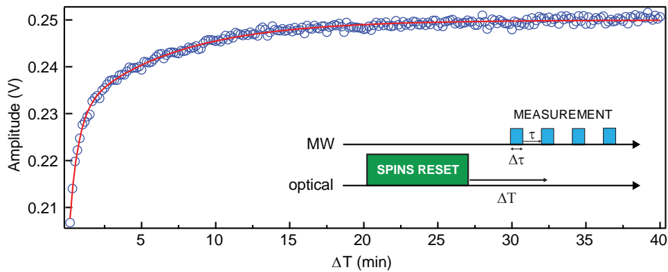
Figure 4.32: NV spin relaxation time . Blue dots are the average reflected amplitude of each probe pulse. A bi-exponential fit (red solid line) yields T_{1,a} = 35 \text{ s} and T_{1,b} = 395 \text{ s} , with respective weights A_{1,a} = -0.022 and A_{1,b} = -0.020 .
