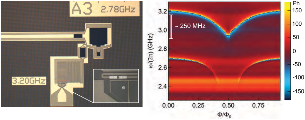
Figure 5.19: Towards a complete silencing of the echo. (left) Fabricated circuit showing the resonators B and TF. The resonator B, to which the spins are coupled, is made in a geometry compatible with the reset operation. It is coupled to the frequency tunable resonator TF by a large coupling capacitance ( C_{B-TF} \sim 300 fF). (right) Reflected phase onto the circuit. A detuning \Delta_B \sim 2\pi \times 250 MHz is achieved at f = 0 .
