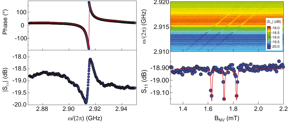
Figure 5.3: Spectroscopy of the system. (left) Reflection spectrum S_{11} of the resonator. The fit of the phase response (red line) yields resonator frequency \omega_r/2\pi = 2.915 GHz and quality factor Q = 650 \pm 100 . (top right) Reflected amplitude |S_{11}| as a function of the applied magnetic field B_{NV} . The three dips characteristic of the NV hyperfine structure are observed. On the bottom, the measured (dots) and computed (line) reflection spectrum at the resonator frequency \omega_r .
