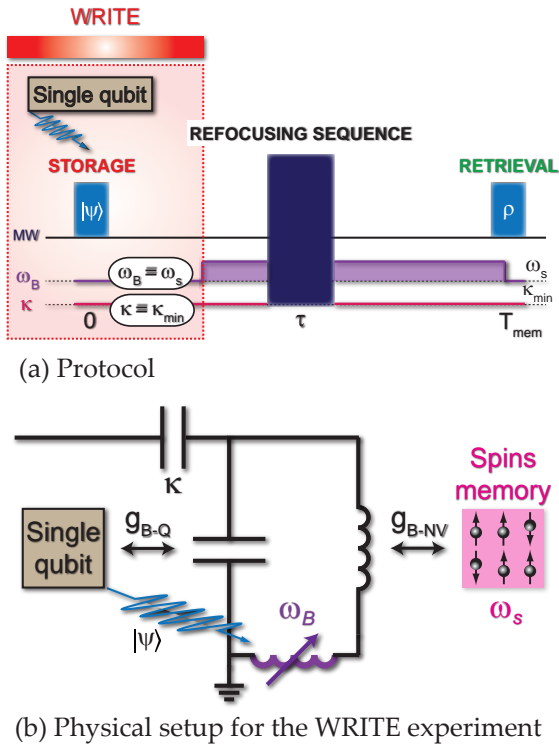
Figure 3.4: Principle of the experiment. (a) Quantum states delivered by a QuP, materialized by a single superconducting qubit, are stored into the spin ensemble. (b) The resonator, with frequency \omega_B tunable and high quality factor, is strongly coupled to both the spin ensemble (frequency \omega_s ) with an ensemble coupling strength g_{B-NV} and a qubit (frequency \omega_Q ) with coupling strength g_{B-Q} . The qubit delivers quantum states to the bus resonator to be stored into the spins memory.
