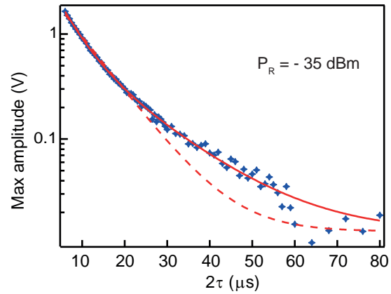
Figure 4.39: Spin echo coherence time T_2 measurement. Measured (crosses) decay of the echo maximum amplitude as a function of \tau . Dashed and solid lines are an exponential fit yielding a characteristic time T_2 = 8.4\mu\text{s} and a bi-exponential fit f(\tau) yielding T_{2A} = 4.7\mu\text{s} and T_{2B} = 14.3\mu\text{s} , respectively.
