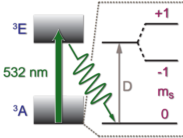
Figure 1.30: Optical repumping of NV centers in their m_S = 0 ground state by application of green (532 nm) laser pulses exciting the {}^3E - {}^3A transition.
