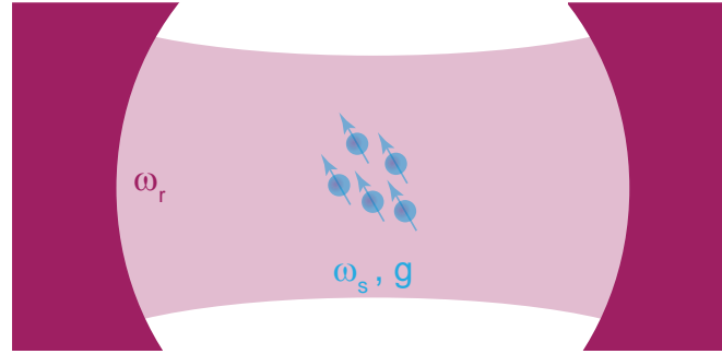
Figure 1.33: The Tavis-Cummings model. N identical two-level systems of frequency \omega_s are identically coupled to a single cavity mode with coupling strength g .
