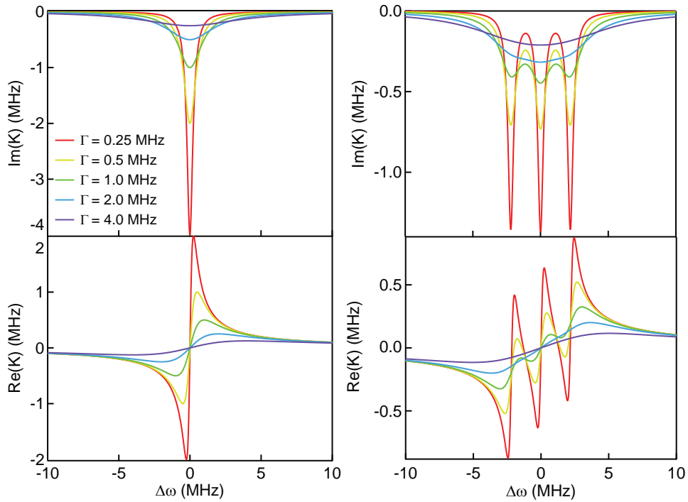
Figure 1.39: The K-function. The imaginary and real part of the function K(\omega) are displayed respectively on the top and on the bottom for a Lorentzian (left) and sum of three Lorentzian (right) distributions.
