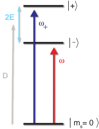
Figure 1.27: Electron spin levels of the electronic ground state.
