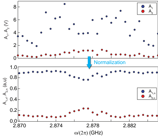
Figure 4.60: Renormalization for comparison to the theory. The fitted A_{i=1,2} (top) are renormalized to 1 (bottom) as A_{i,n} = A_i / (\sum_i A_i) for i = 1, 2 .
