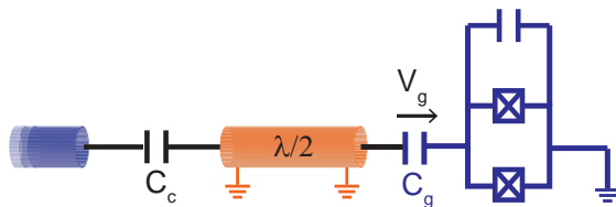
Figure 1.20: Schematic of a typical CQED circuit, consisting of a Transmon qubit capacitively coupled to a transmission line resonator.
