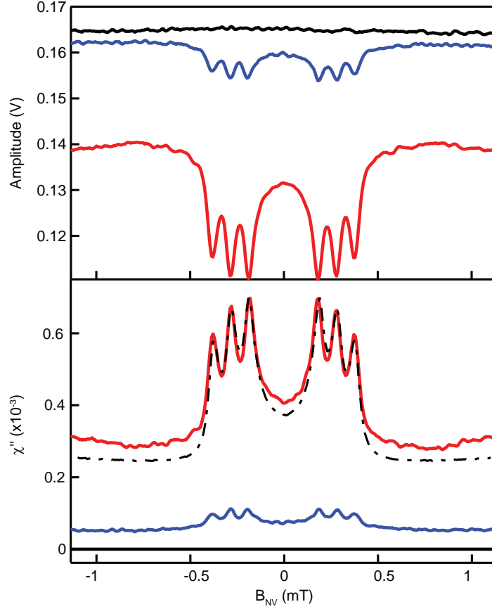
Figure 4.28: Polarization of the spins with an optical pulse. The signal of the spins after an optical pulse of power P_L = 1.47 \text{ mW} and duration T_L = 4 \text{ s} (red line) is compared to the one at equilibrium (blue line) and saturated (black line). (top) Reflected amplitude. The curves show the hyperfine split m_S = 0 to m_S = \pm 1 spectroscopic transitions of the N-Orth sub-ensemble. (bottom) Corresponding imaginary part \chi''(B_{NV}) of the spin susceptibility. The calculated spin susceptibility (see Appendix B) and rescaled by a global factor to match the experimental spin polarization is shown (dash-dotted line).
