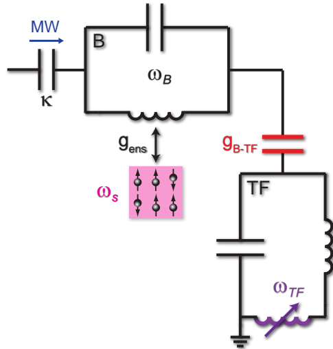
Figure 5.10: Schematic of the circuit. The main resonator, with frequency \omega_B and damping rate \kappa , is coupled to the spin ensemble (frequency \omega_s ) with a coupling constant g_{\text{ens}} . It is strongly coupled with strength g_{B-TF} to a second resonator with frequency \omega_{TF} .
