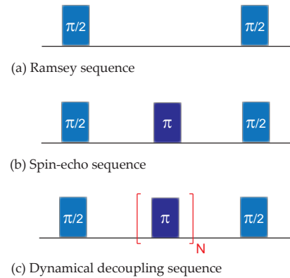
Figure 1.31: Measuring the coherence times. (a) Ramsey sequence. Two \pi/2 rotations are performed, separated by a delay during which the spins precess freely. The envelope of the oscillations for increasing \tau is characterized by the dephasing time T_2^* , associated to fluctuations of the environment. (b) Spin echo sequence. An intermediate \pi rotations around x is performed to refocus the dephasing due to static fluctuations. (c) Dynamical decoupling sequence. Successive \pi rotations are performed to refocus the dephasing due to dynamic fluctuations.
