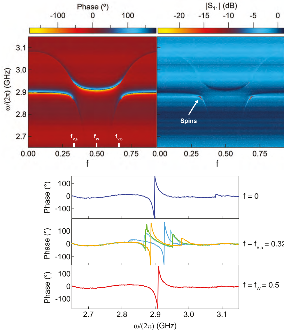
Figure 5.12: Reflection spectrum S_{11} of the circuit. Reflected phase (top left) and amplitude (top right) as a function of the applied flux f = \Phi/\Phi_0 , at B_{\text{NV}} = 0 mT. Two f -dependent resonances are visible, showing successive anticrossings at f_{V,a} = 0.32 and f_{V,b} = 0.67 . The reflected phase at f = 0, f_{V,a}, f_W is plotted in the bottom panel.
