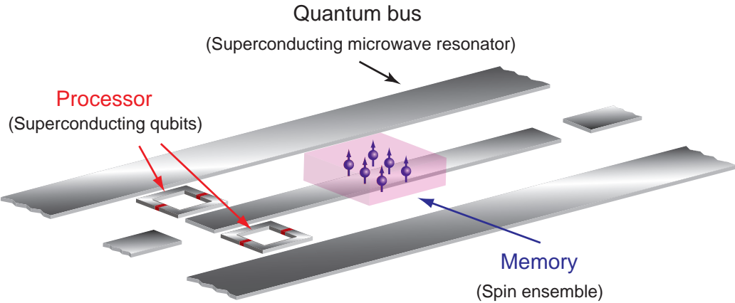
Figure 2: Concept of the hybrid quantum processor combining a few(2)-qubits processor and a spin ensemble multimode quantum memory. The microwave photon exchange between both is implemented by a superconducting resonator used as a quantum bus, which is coupled electrically to the qubits and magnetically to the spins.
