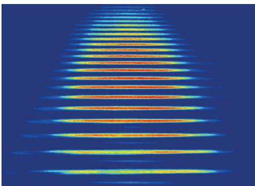
Spectrum of a beam of high-order harmonics of the laser frequency produced by a relativistic plasma mirror driven by a 100TW femtosecond laser pulse experiments with UHI100 laser @ CEA Saclay)
