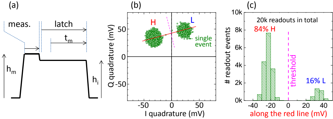
Figure 4.5: a) Microwave pulse envelope used for exciting the CJBA at readout. The pulse consists of a measurement part with amplitude h_m and a latching part with amplitude h_l = 0.8 - 0.9h_m . To determine the state of the resonator during the latching interval, the quadratures I and Q of the reflected signal are averaged over the time window t_m . b) Bimodal distribution of the time-averaged (I, Q) values obtained for a readout power close to the bifurcation threshold. The red dotted line perpendicular to the principal axis joining the two modes of the distribution and going through the mean quadratures (I_0, Q_0) provides an optimal separation between the two clusters corresponding to the L and H states. c) Histograms of the signal projected on the principal axis (red line), revealing a switching probability of 84% for the example shown.
