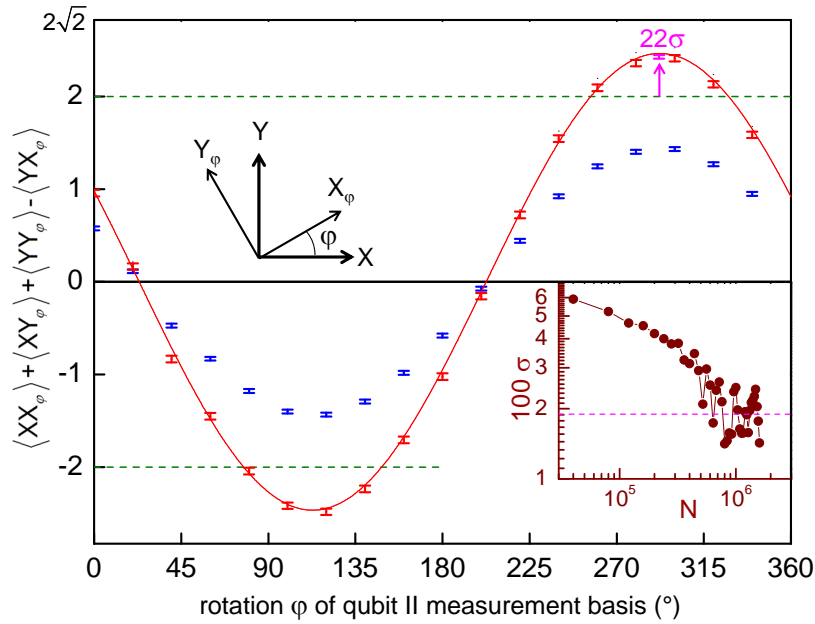
Figure 1.6: Measured average value of the CHSH operator for a prepared Bell state. After readout error corrections, the CHSH expectation value (red points) exceeds the classical boundary of 2 . The raw measurement data (blue points) lies below this critical threshold. The inset shows the standard deviation \sigma at the highest point of the curve as a function of the measurement sample size. For the highest sample count, the classical boundary is exceeded by 22 standard deviations.
