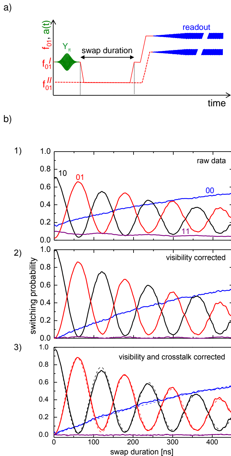
Figure 5.6: a) Pulse sequence used to create an entangled two-qubit state using a non-adiabatic pulse that brings the qubits in resonance for a well-defined time. b) State occupation probabilities for the two-qubit register during a coherent energy swap. b1) Shows the raw state probabilities corresponding to the states |00\rangle , |01\rangle , |10\rangle and |11\rangle , b2) shows the same data corrected for the limited visibility of each qubit readout and b3) shows the fully corrected readout probabilities where we account for both visibility and inter-qubit readout crosstalk errors.
