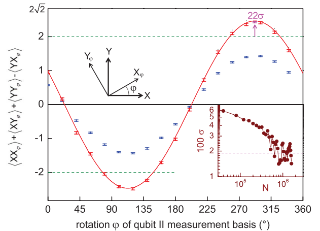
FIG. 3 (color). Test of the CHSH-Bell inequality on a |10\rangle + e^{i\psi}|01\rangle state by measuring the qubits along X^I or Y^I and X^{II}_\phi or Y^{II}_\phi (see top-left inset), respectively. Blue (red) error bars are the experimental CHSH entanglement witness determined from the raw (readout-error corrected) measurements as a function of the angle \phi between the measuring basis, whereas solid line is a fit using \psi as the only fitting parameter. Height of error bars is \pm 1 standard deviation \sigma(N) (see bottom-right inset), with N the number of sequences per point. Note that averaging beyond N = 10^6 does not improve the violation because of a slow drift of \phi .
