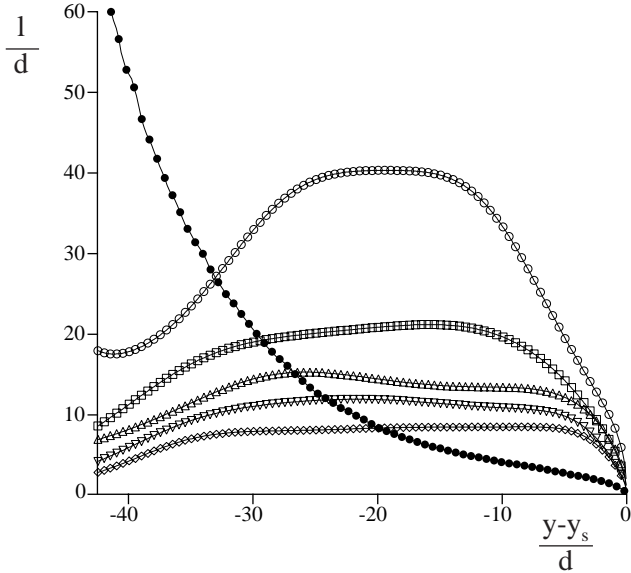
Fig. 9. Correlation length l(y) obtained from inclined plane simulations IP4 for \theta = 15^\circ (○), \theta = 16^\circ (□), \theta = 17^\circ (△), \theta = 18^\circ (▽), \theta = 21^\circ (◇), and from heap case experiment SF4 (●).
