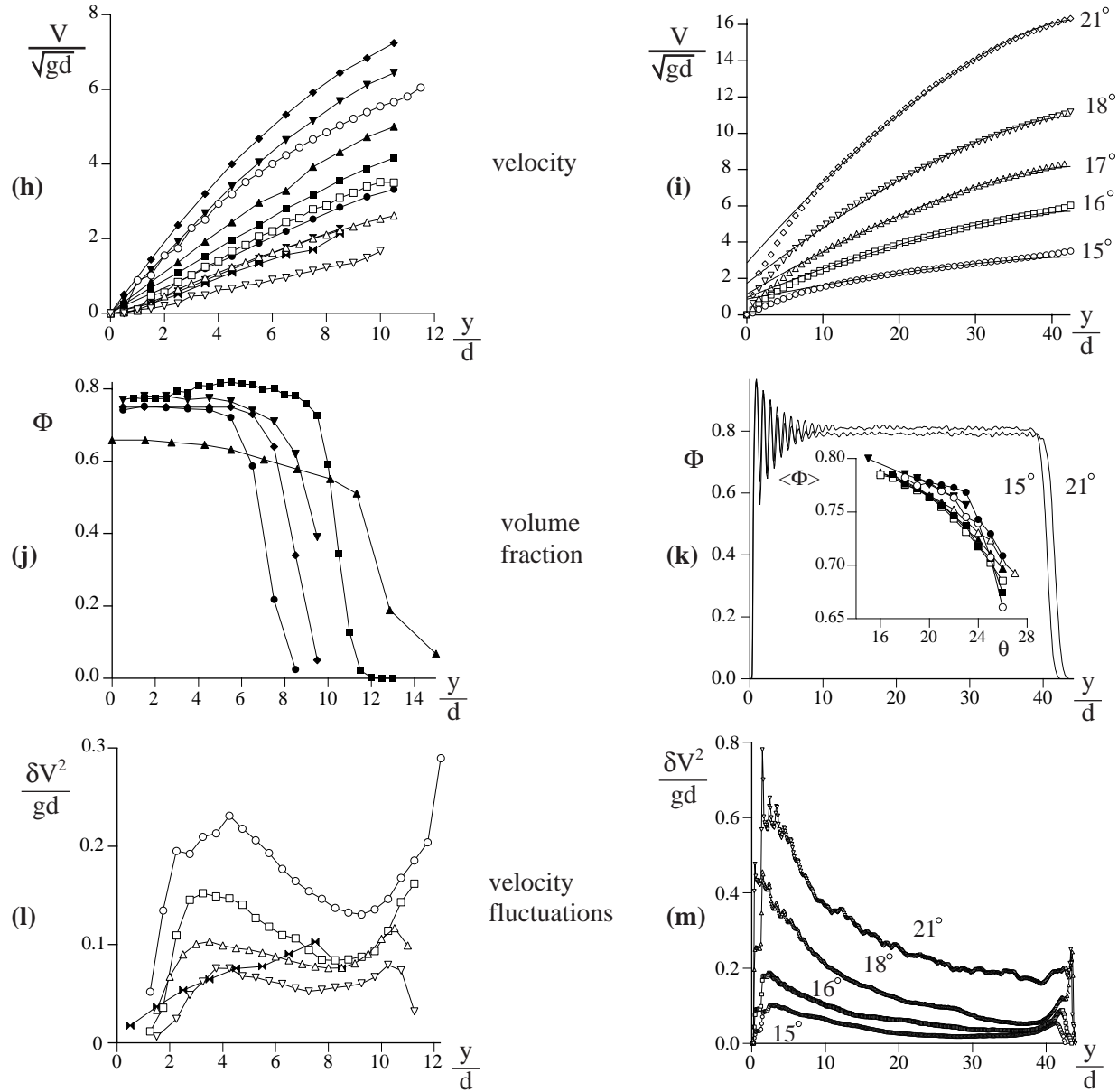
Fig. 5. Rough inclined plane. (h) Velocity profiles for thin flows from experiment IP2 for \theta = 34^\circ, 36^\circ (black bow ties), IP1 for \theta = 21^\circ ( \bullet ), 22^\circ ( \blacksquare ), 23^\circ ( \blacktriangle ), 25^\circ ( \blacktriangledown ), 27^\circ ( \blacklozenge ), and simulations IP4 ( e=0.6 ) with \theta = 12.6^\circ ( \nabla ), 14.4^\circ ( \triangle ), 16.2^\circ ( \square ), 18^\circ ( \circ ); (i) Velocity profiles for thick flows from numerical simulations IP3. (j) Volume fraction profiles for thin layers from simulations IP4 ( e = 0.7 ) for \theta = 14.4^\circ , ( \blacksquare ), IP3 for \theta = 23^\circ ( \blacklozenge ), from experiments IP2 for \theta = 34^\circ ( \bullet ), IP1 for \theta = 22^\circ ( \blacktriangledown ), IP9 for \theta = 27^\circ ( \blacktriangle ); (k) Volume fraction profiles for thick flows from simulation IP3; Inset: mean volume fraction versus inclination angle for different flow thickness; (l) Velocity fluctuations profiles for thin layers from experiment IP2 for \theta = 34^\circ (black bow ties) and from simulations IP4 ( e = 0.6 ) for \theta = 12.6^\circ ( \nabla ), \theta = 14.4^\circ ( \triangle ), \theta = 16.2^\circ ( \square ) and \theta = 18^\circ ( \circ ); (m) Velocity fluctuations profiles for thick layers from simulations IP3.
