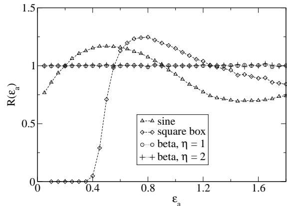
FIG. 1: Ratio R(\varepsilon_a) of forward and backward probabilities of a transition path; R(\varepsilon_a) \neq 1 indicates a breaking of detailed balance. Distributions \psi(q) used are the sine-like distribution ( \Delta ) and the ‘square box’ one ( \diamond )—see text for details. Results for beta \psi(q) with \eta = 1 ( \circ ) and \eta = 2 ( + ) are also presented for comparison, showing as expected that detailed balance is satisfied for these distributions.
